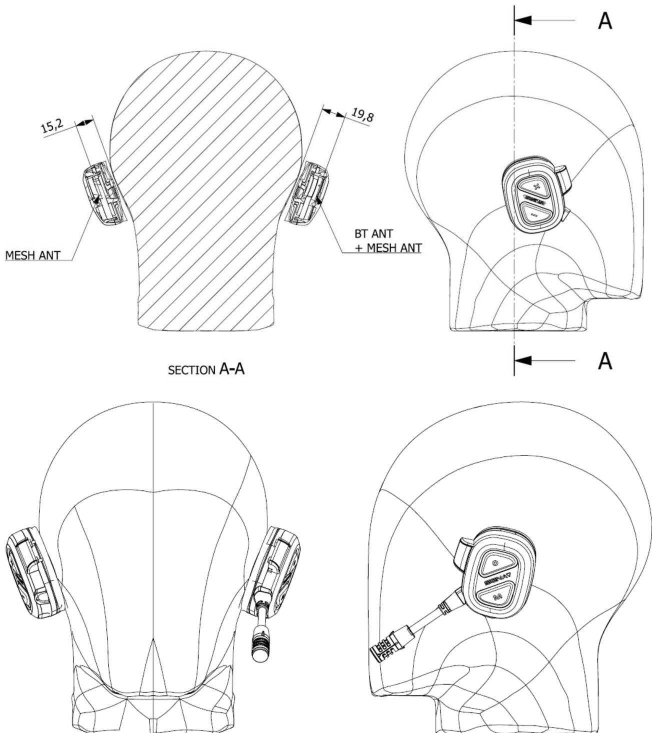
Figure E-1 Antenna Location
