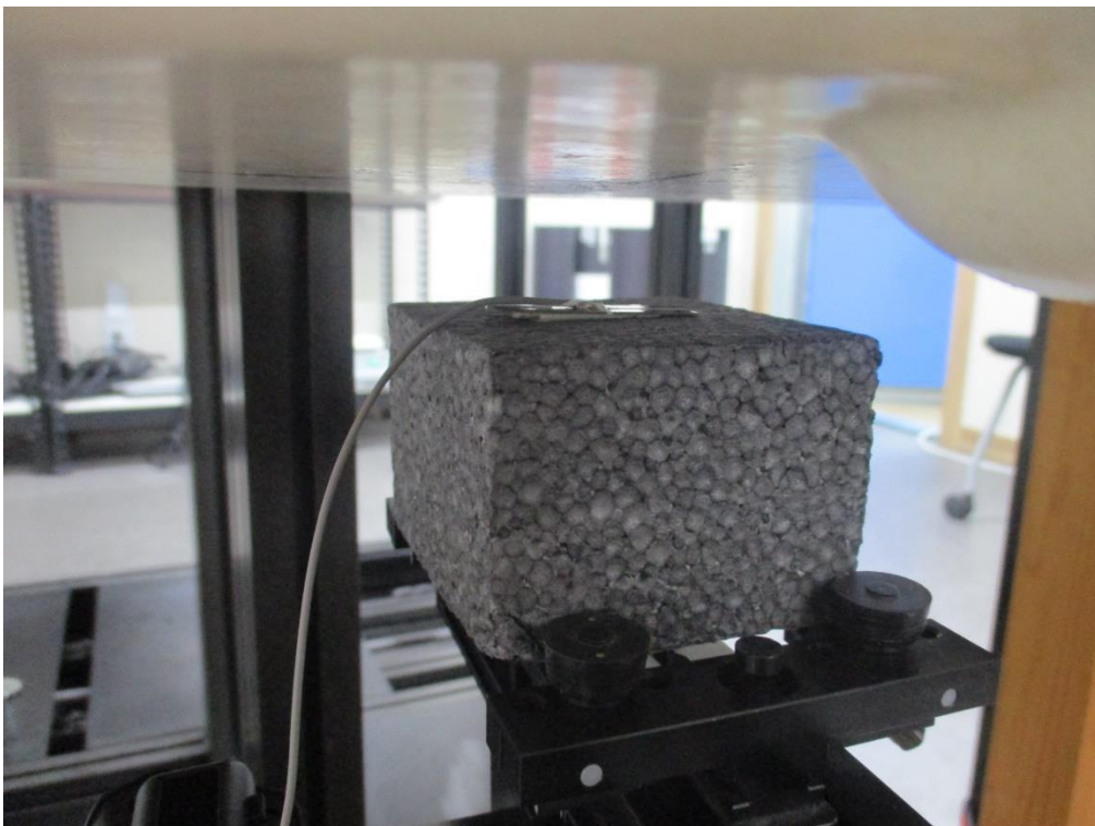
Rear Side from Flat Phantom (Separation Distance: 2 cm) – Head SAR
