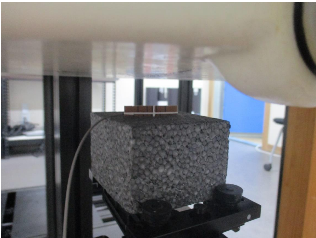
Left Side from Flat Phantom (Separation Distance: 2 cm) – Head SAR
