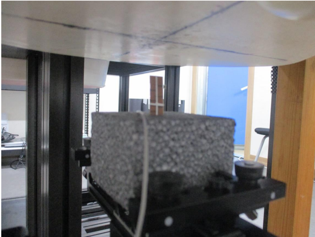
Top Side from Flat Phantom (Separation Distance: 2 cm) – Head SAR
