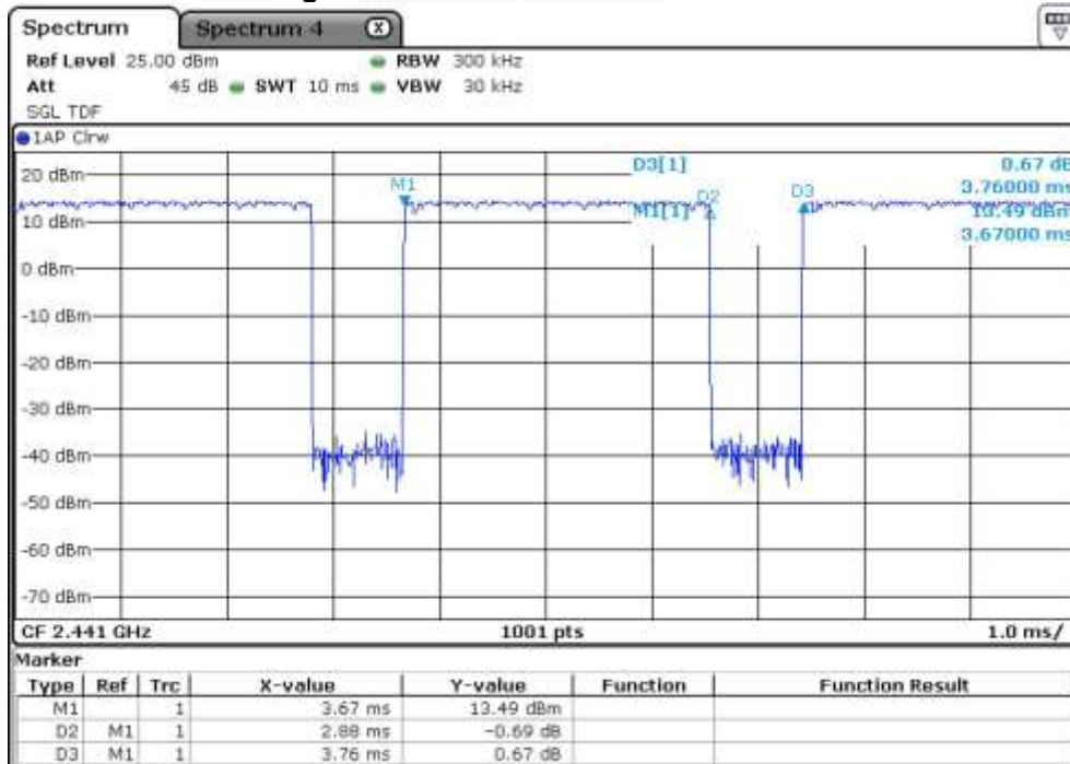
Figure 7-1 Bluetooth Transmission Plot
