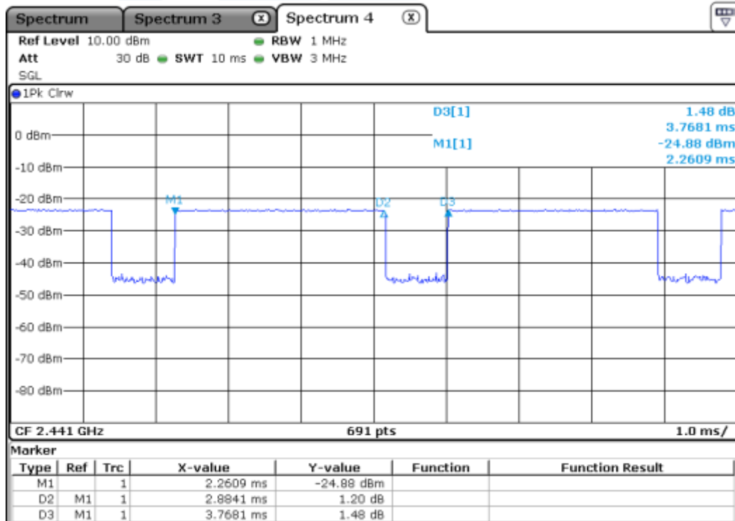
Figure 7-2 Bluetooth(QCC) Transmission Plot
