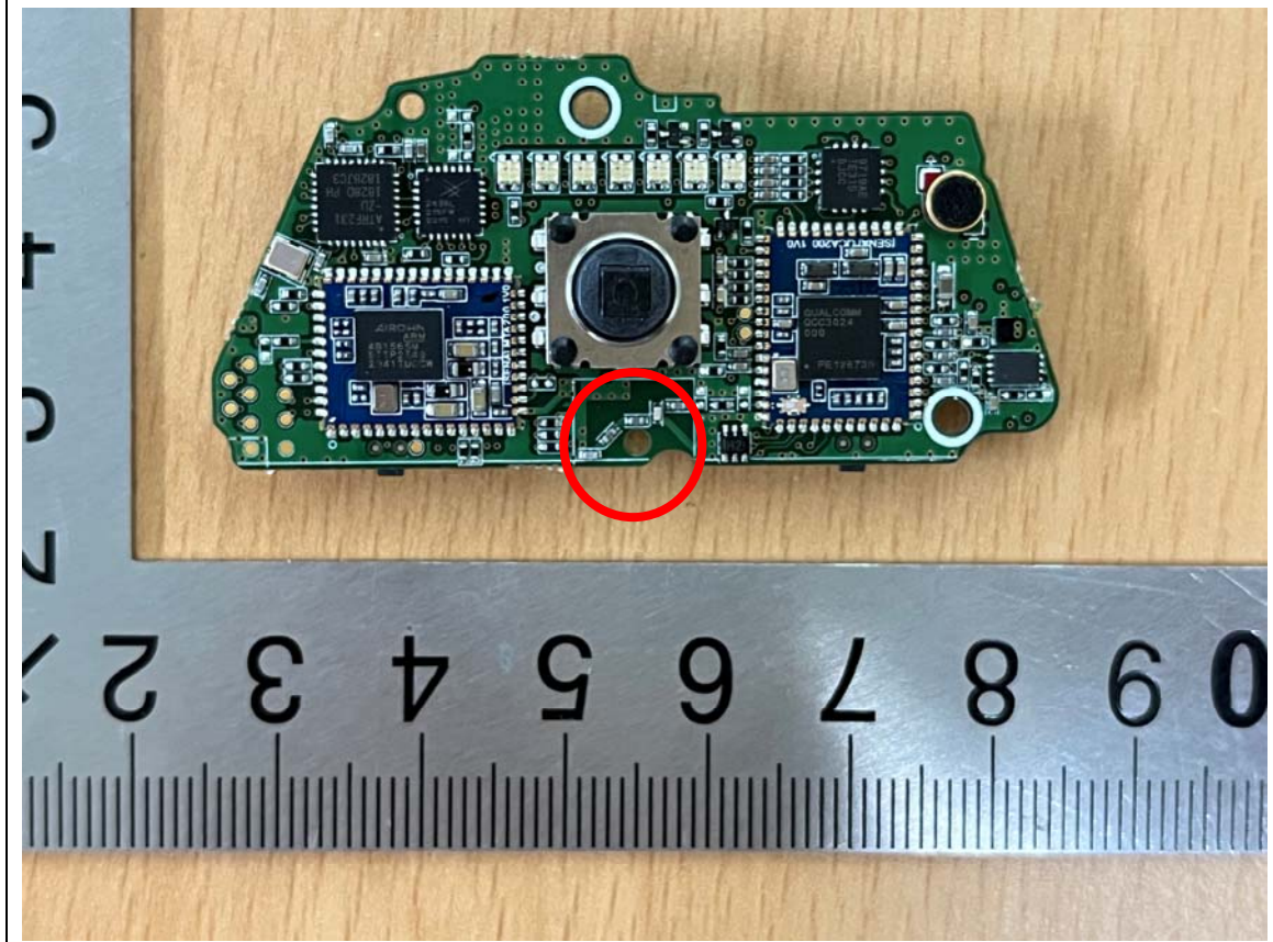
BT Antenna
