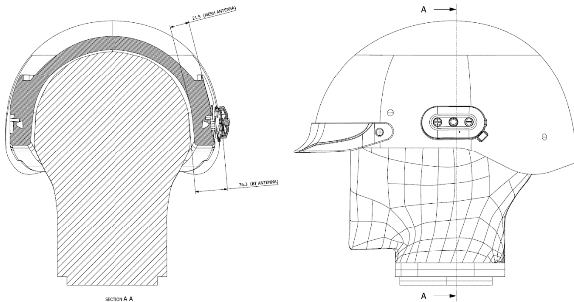
Figure E-1 Antenna Location
