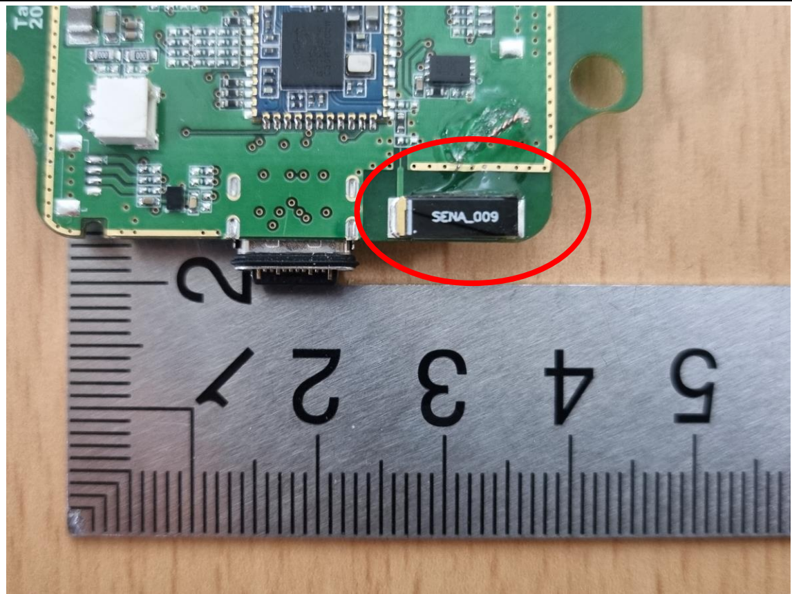
BT Antenna (M/N: SENA_009)
