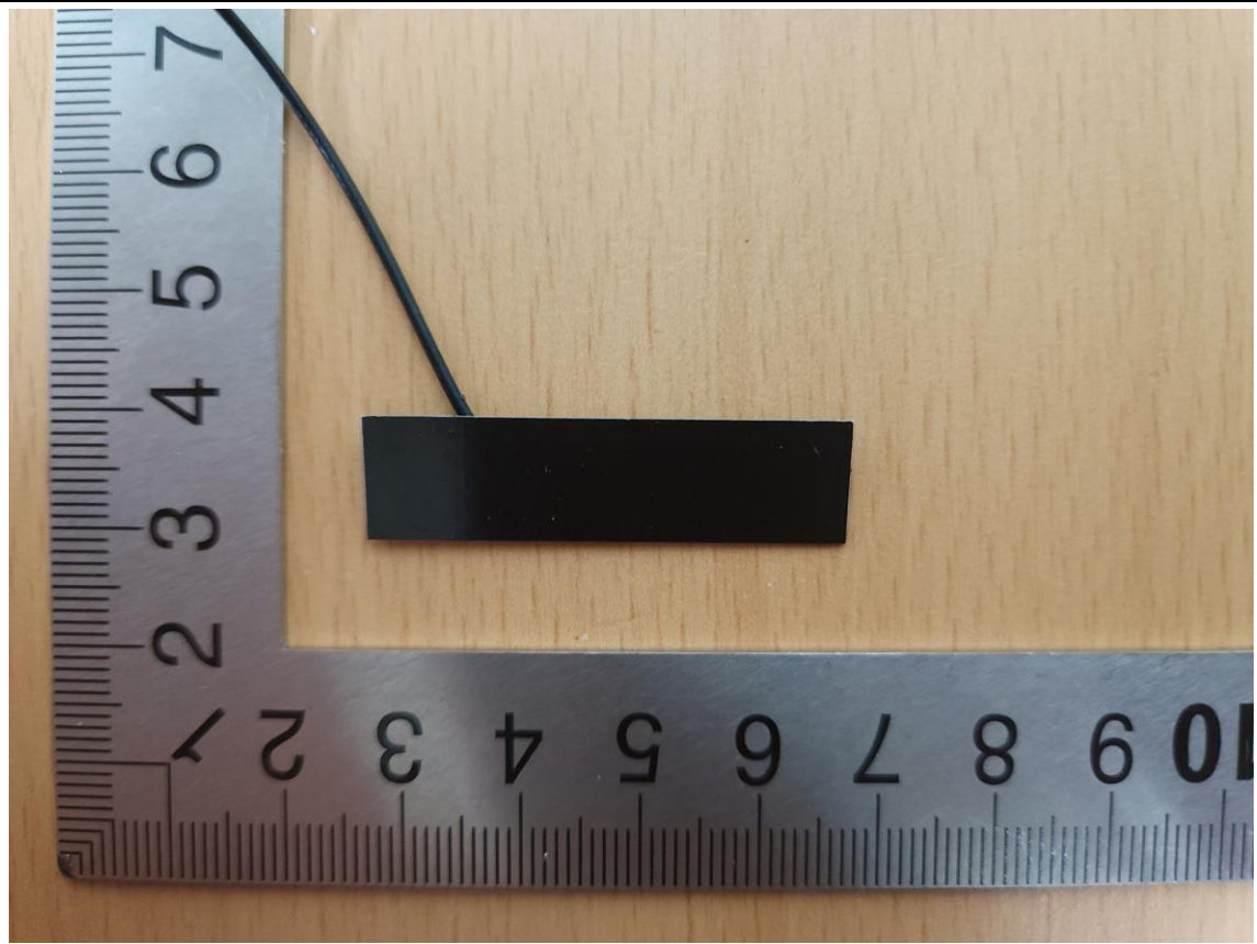
MESH Antenna 2 (M/N: SENA_10A)
