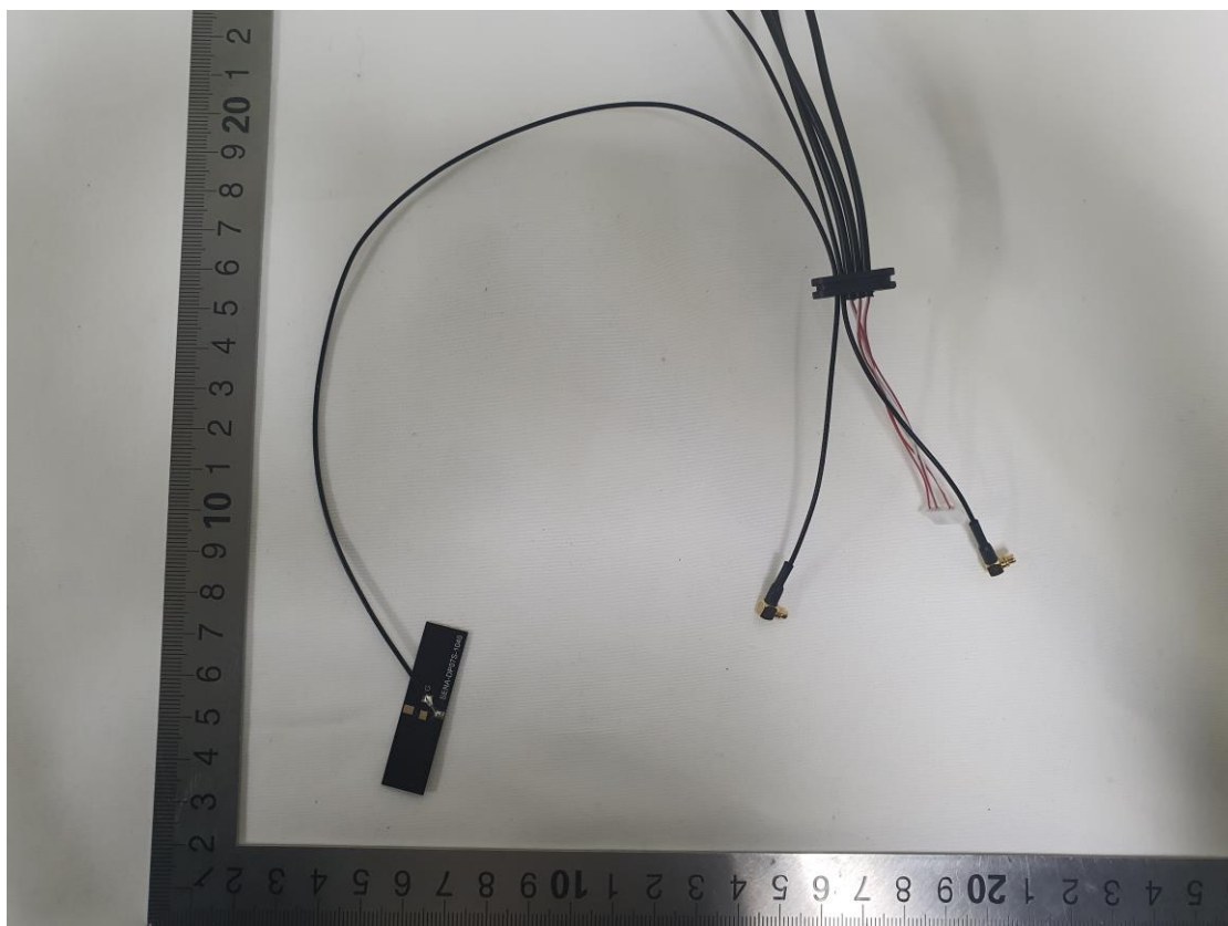
MESH Antenna 2
