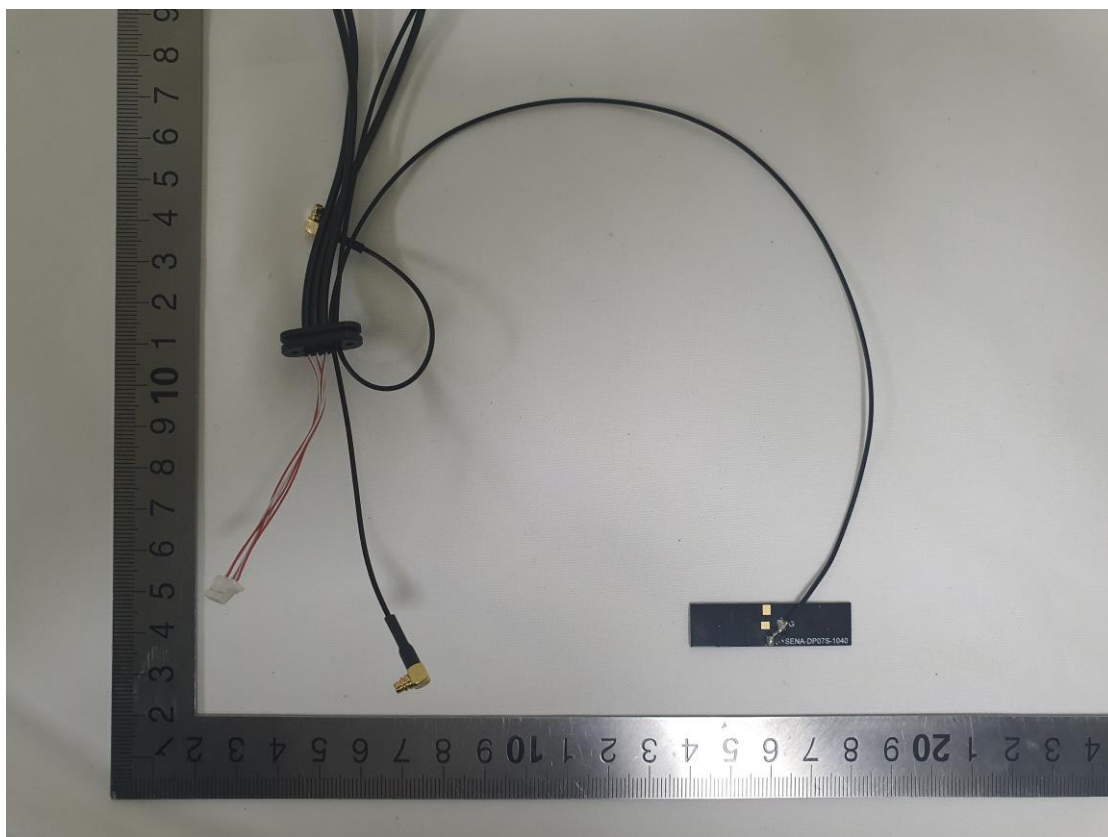
MESH Antenna 1
