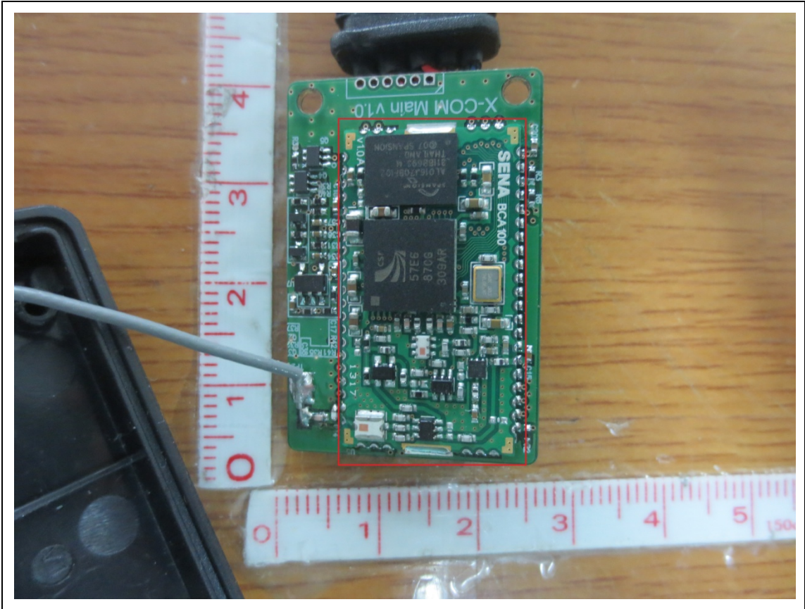
Only RF Module Top View
