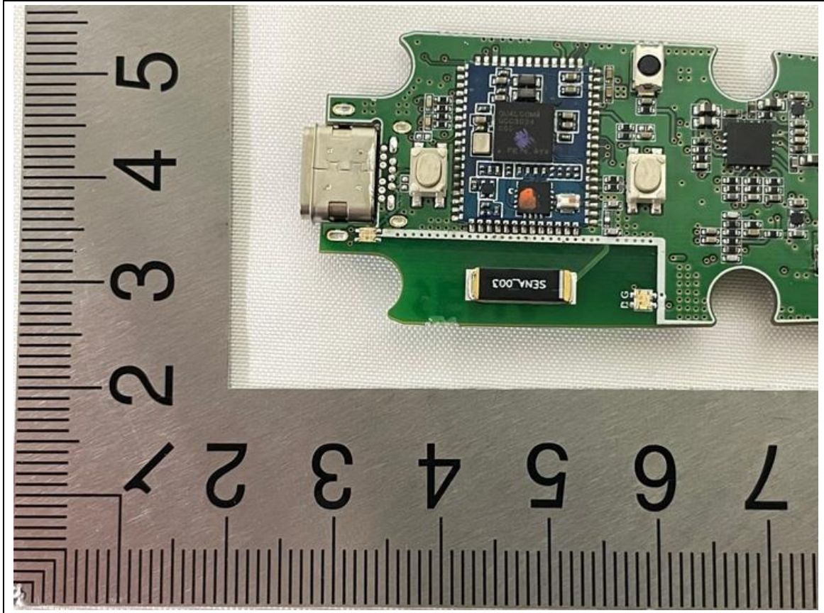
BT Antenna
