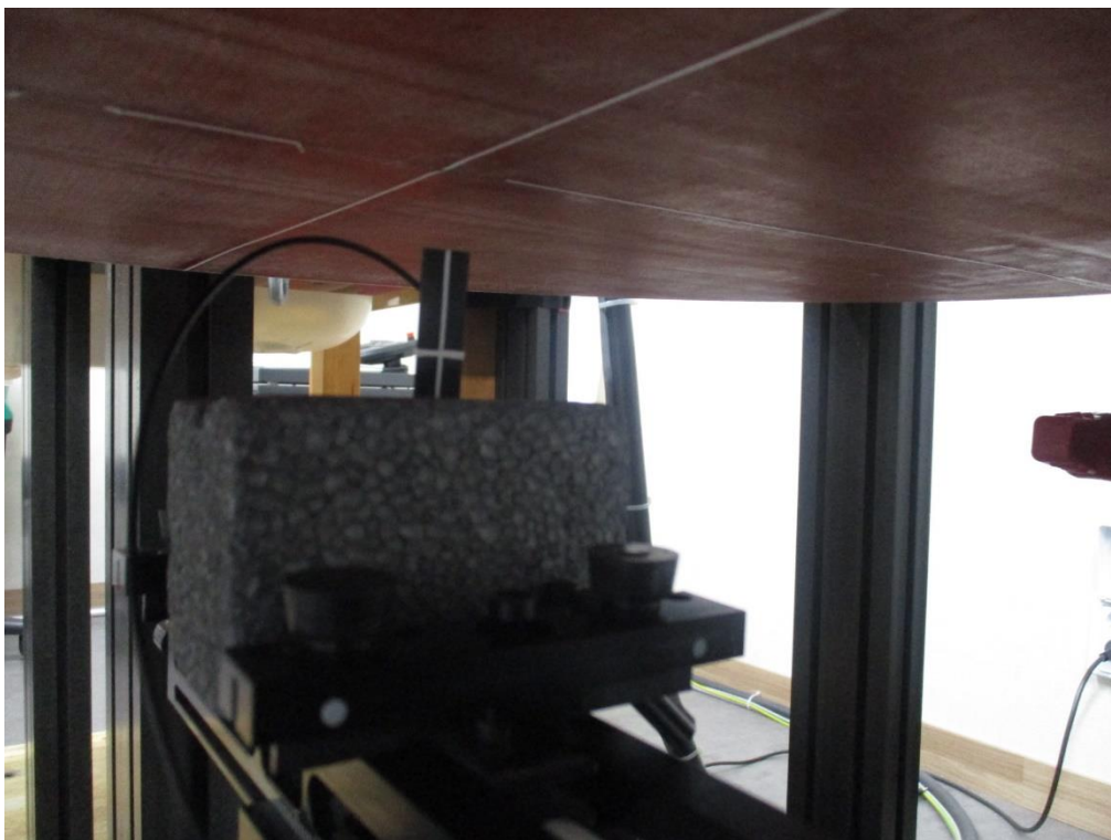
Bottom Side from Flat Phantom (Separation Distance: 1.5 cm) – Bluetooth Antenna
