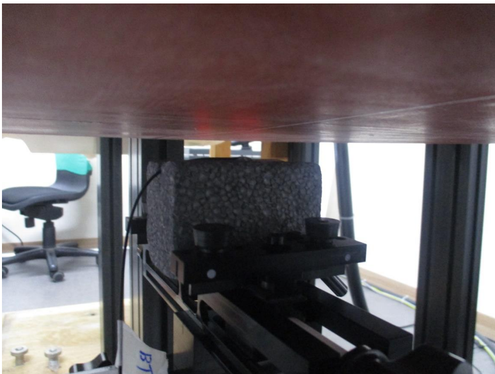
Rear Side from Flat Phantom (Separation Distance: 1.5 cm) – MESH Antenna
