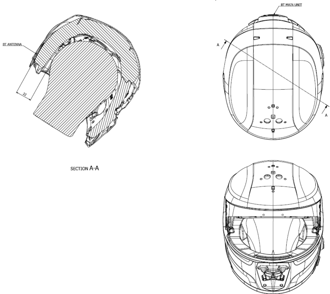
Figure E-1 Antenna Location
