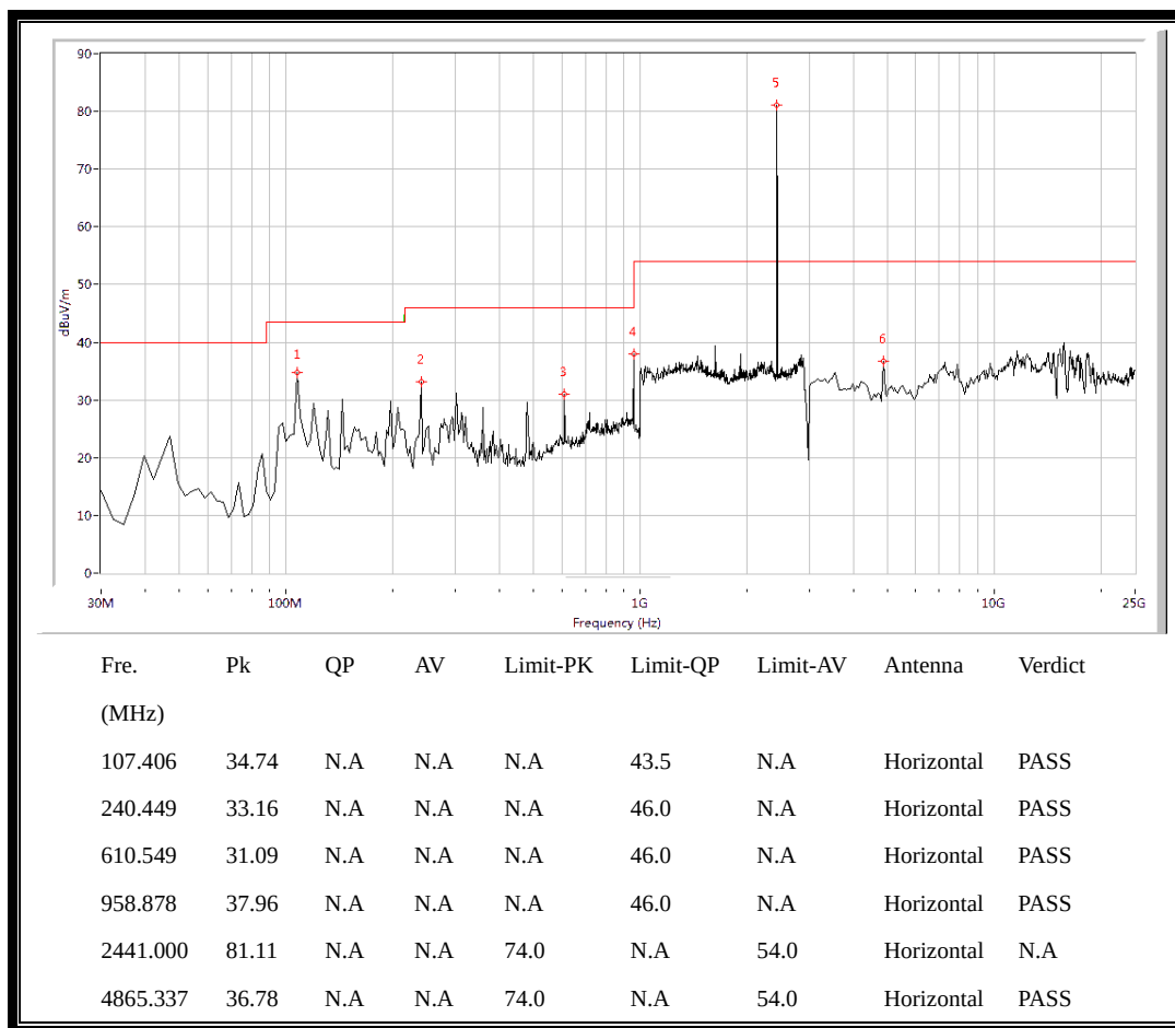
(Plot B.1: 30MHz to 25GHz, Antenna Horizontal @ GFSK, channel 39)
