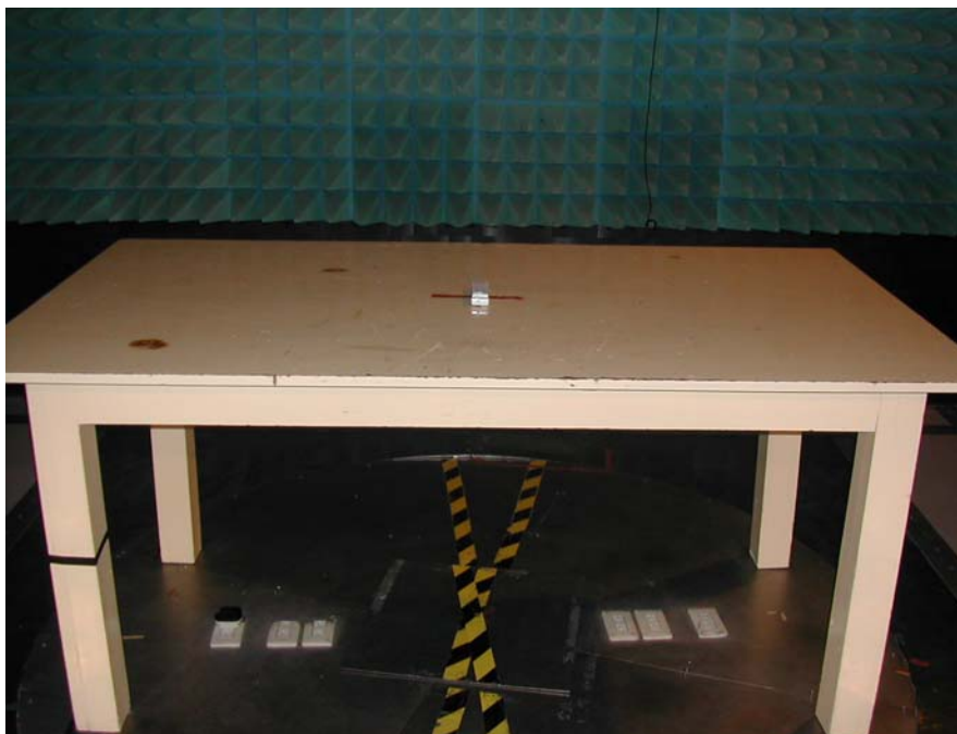
Fundamental & Harmonics Strength Test Set-up Front View
