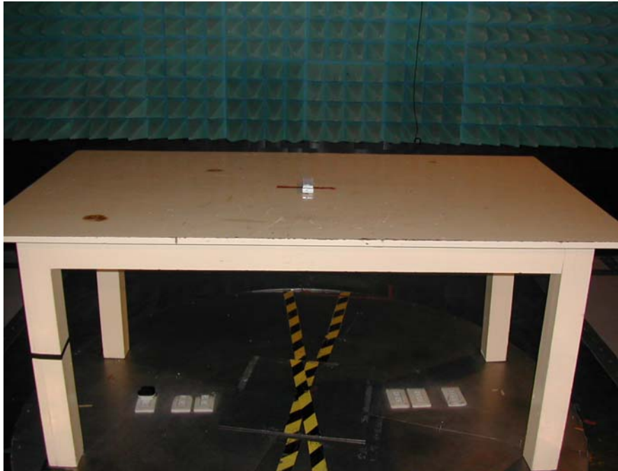
Band Edge Test Set-up Front View
