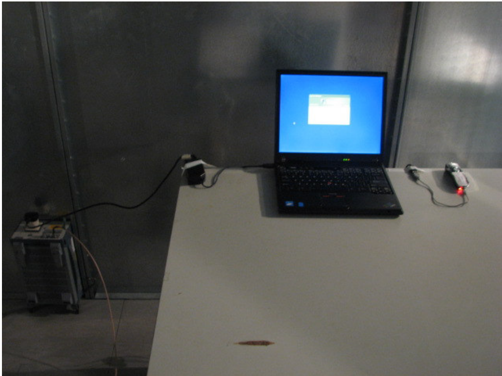
Set-up for Disturbance Voltage on AC Mains (Transceiver)
