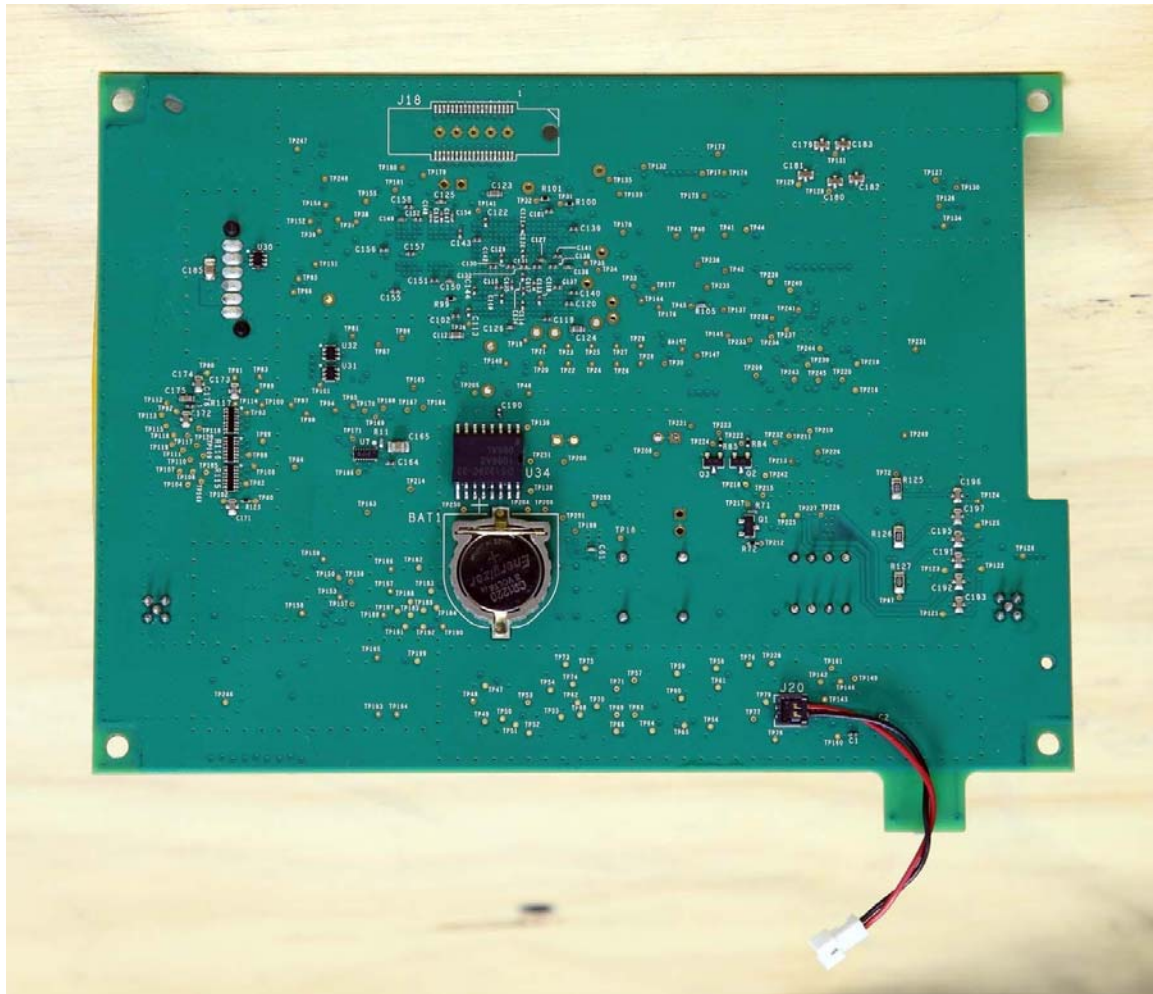
Solder Side
