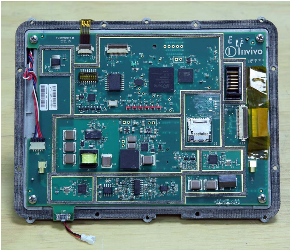
Component Side
