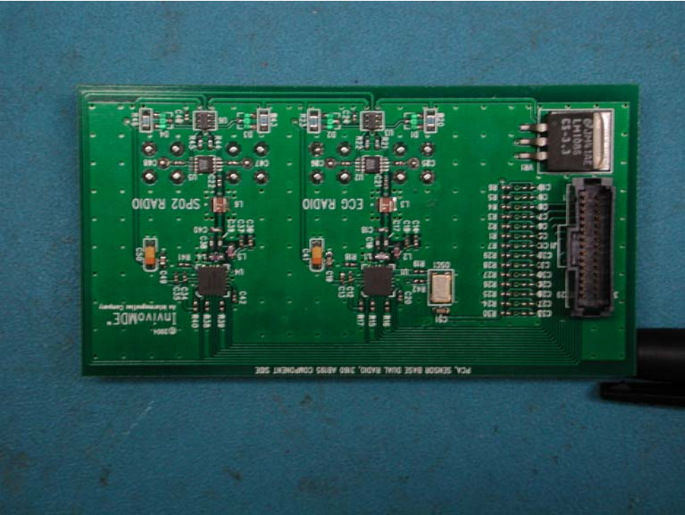
CIRCUIT BOARD
