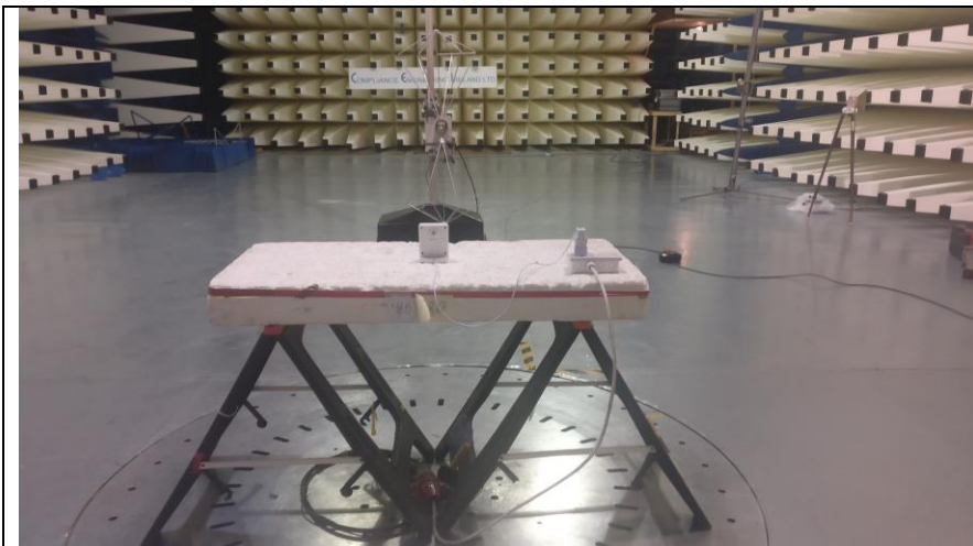
Fig 1b Test setup 30MHz -300MHz Rad Emissions
