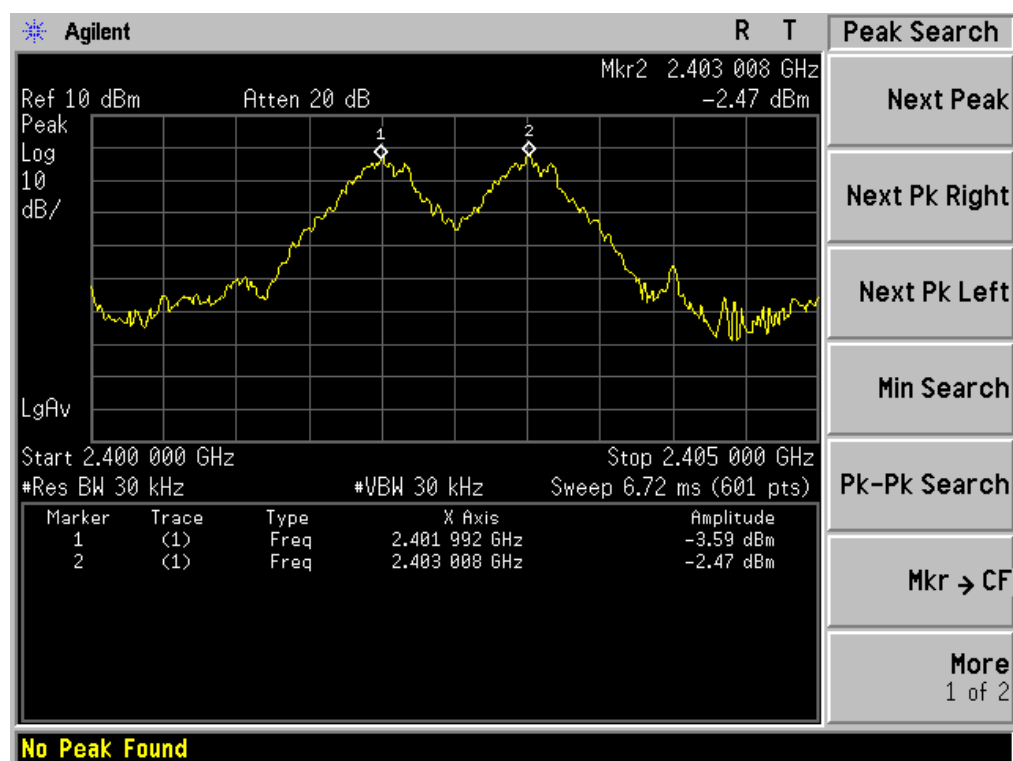
TEST PLOT FOR FREQUENCY SEPARATION ( 1Mbps )
