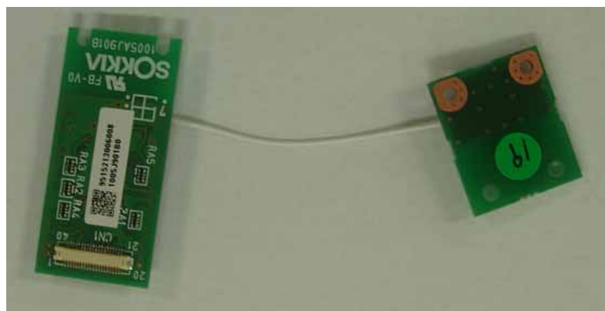
Fig2. Lower view
