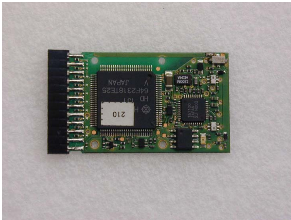
BlueStick-Top (Cover off)
