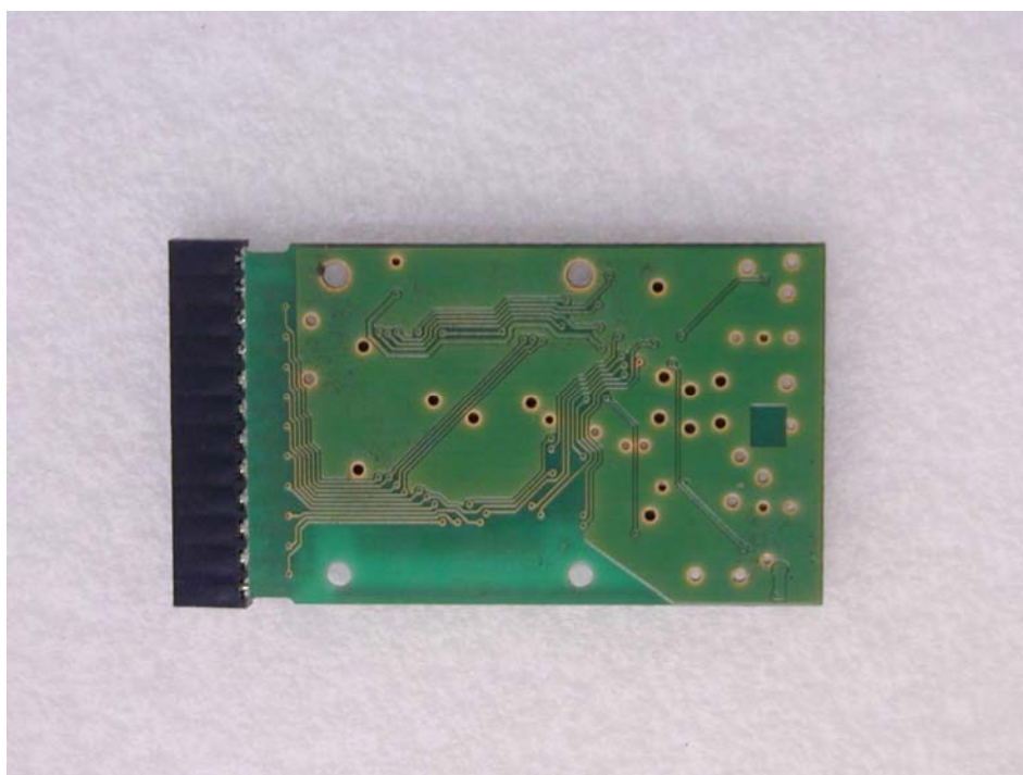
BlueStick-Bottom (Cover off)
