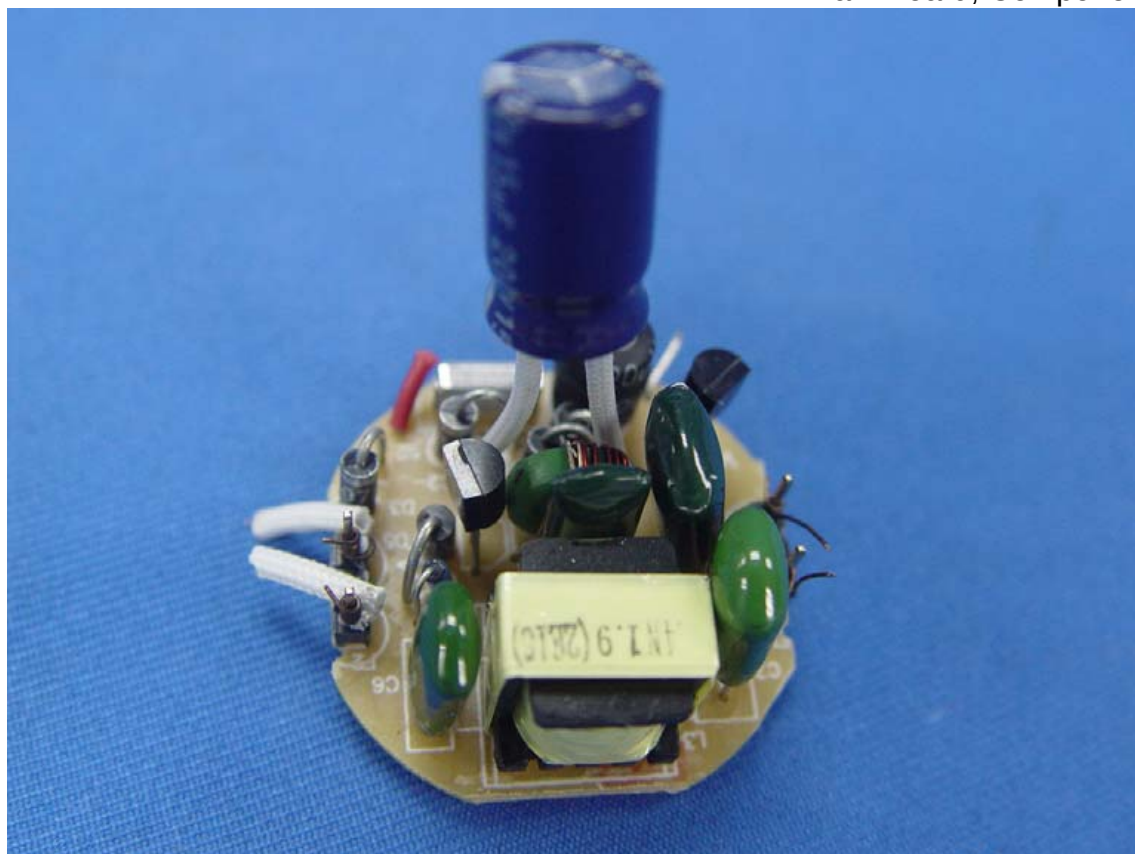
Figure 24 Main Board, Component Side
