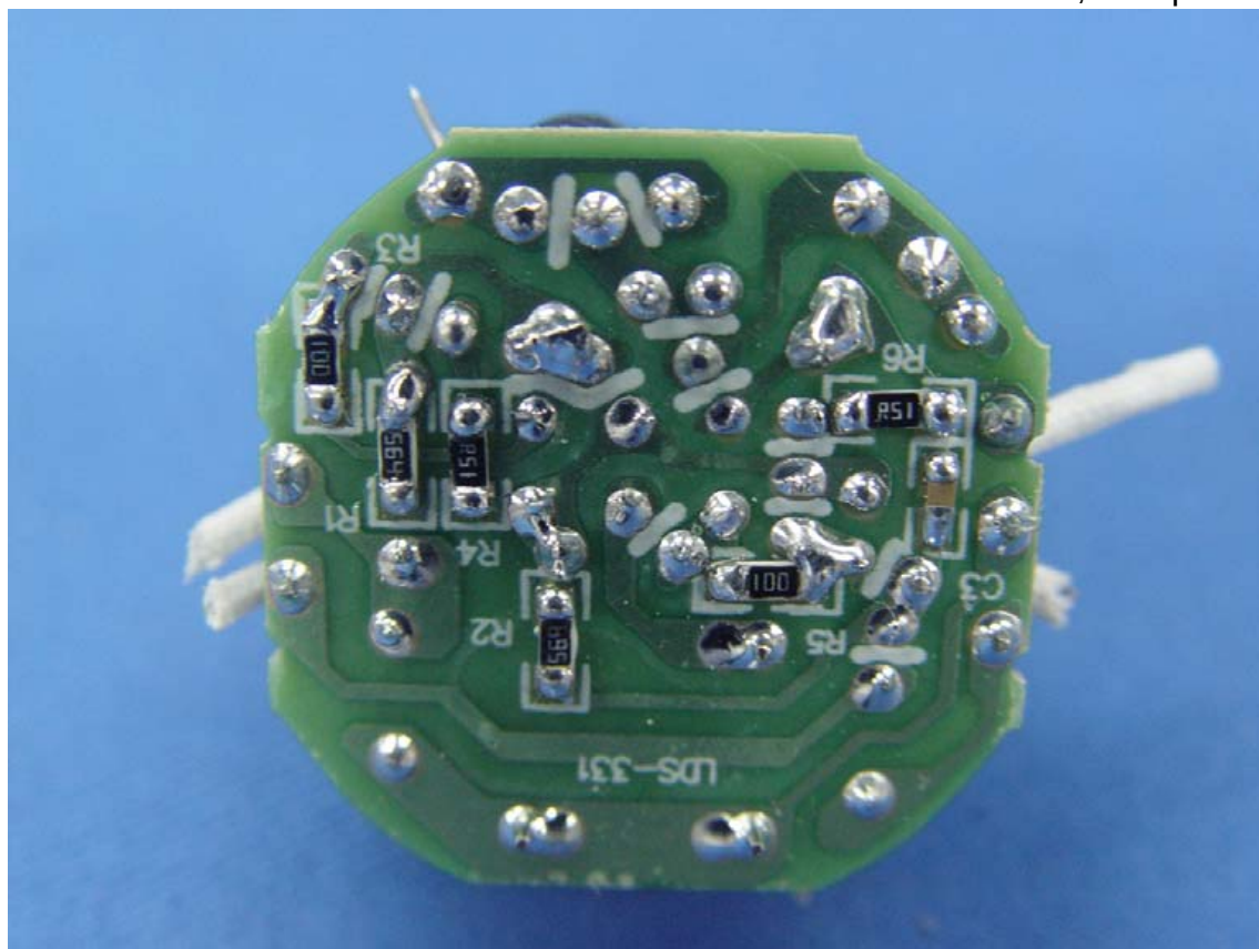
Figure 19 Main Board, Component Side
