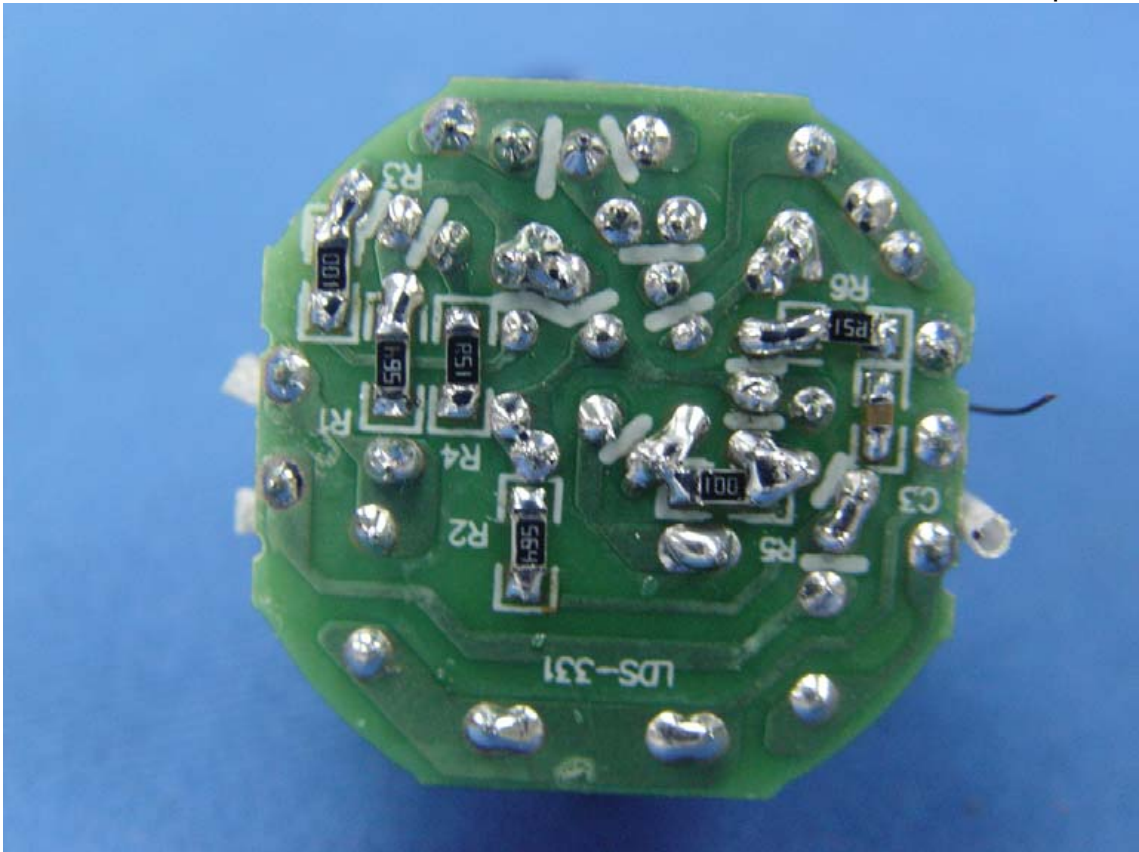
Figure 22 Main Board, Component Side
