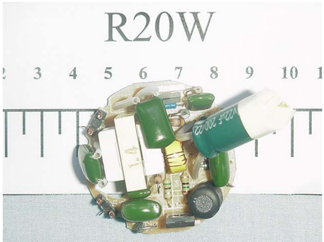
FIGURE 7 ENERGY SAVING LAMP (M/N: R20W) MAIN BOARD (COMPONENT SIDE)
