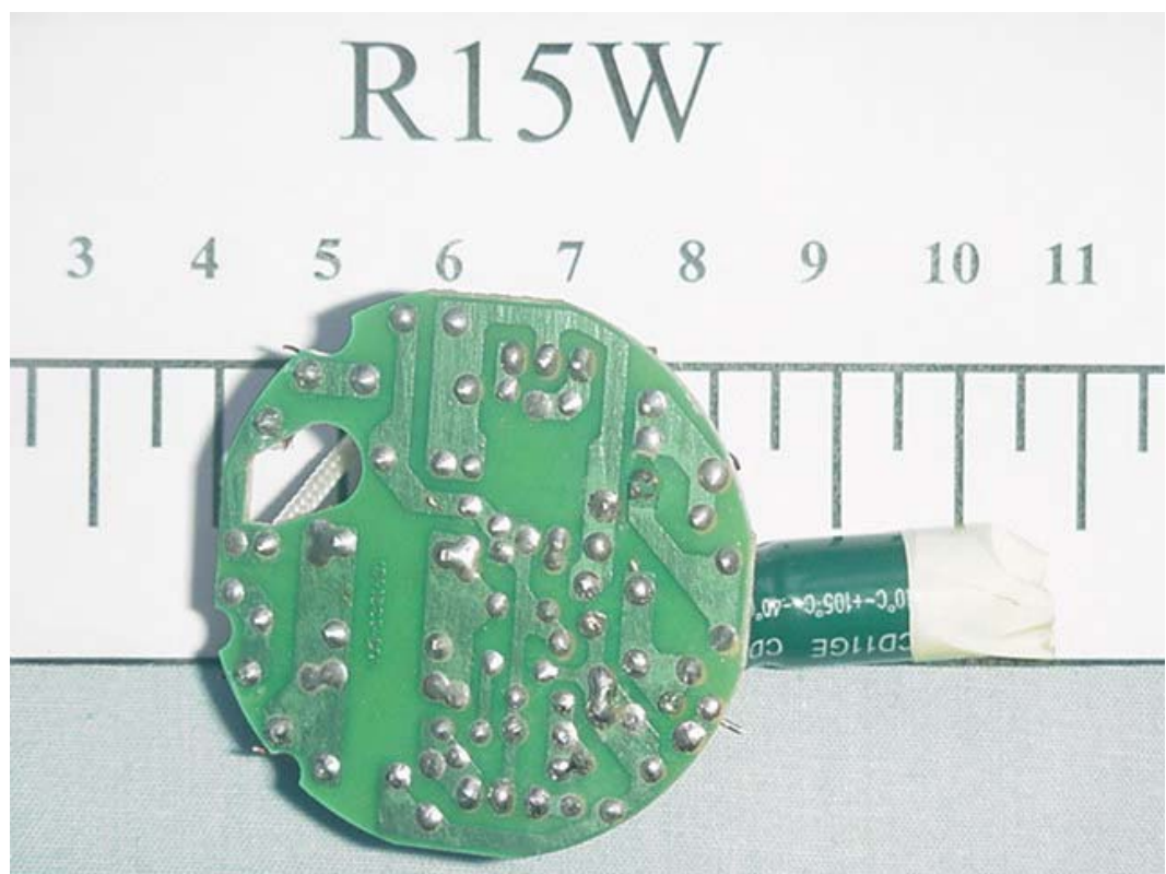
FIGURE 4 ENERGY SAVING LAMP (M/N: R15W) MAIN BOARD (SOLDERED SIDE)
