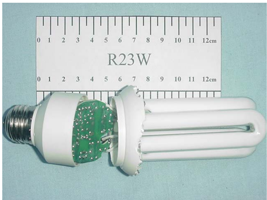
FIGURE 10 ENERGY SAVING LAMP (M/N: R23W) COVER REMOVED 2
