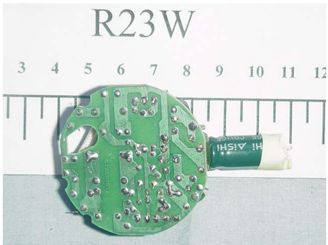
FIGURE 12 ENERGY SAVING LAMP (M/N: R23W) MAIN BOARD (SOLDERED SIDE)
