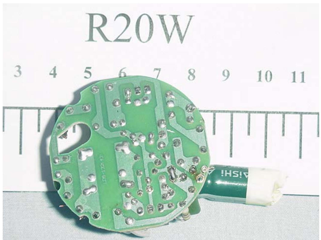
FIGURE 8 ENERGY SAVING LAMP (M/N: R20W) MAIN BOARD (SOLDERED SIDE)
