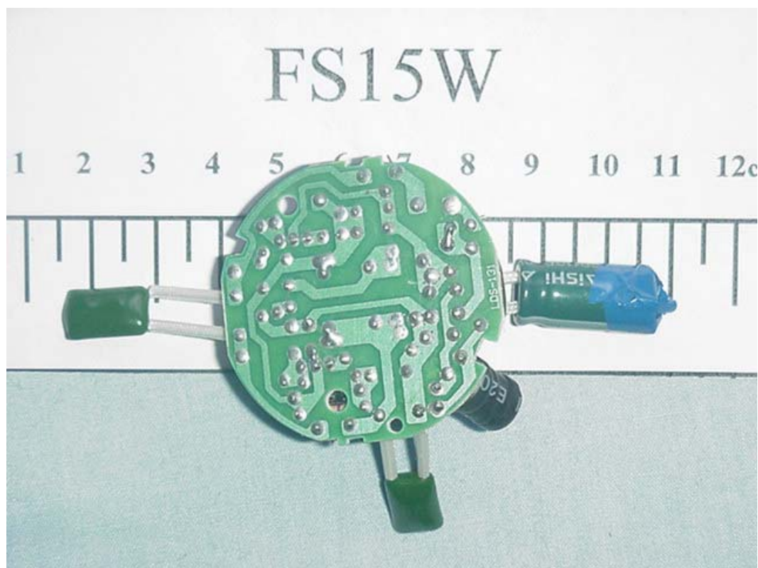
FIGURE 3 ENERGY SAVING LAMP (M/N: FS15W) MAIN BOARD (SOLDERED SIDE)
