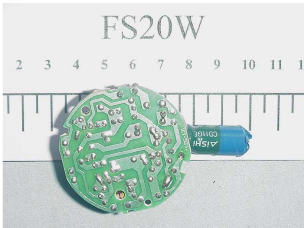
FIGURE 6 ENERGY SAVING LAMP (M/N: FS20W) MAIN BOARD (SOLDERED SIDE)
