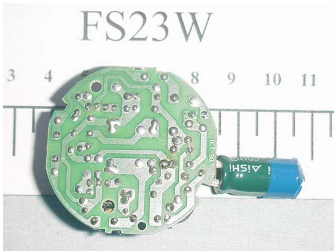
FIGURE 9 ENERGY SAVING LAMP (M/N: FS23W) MAIN BOARD (SOLDERED SIDE)
