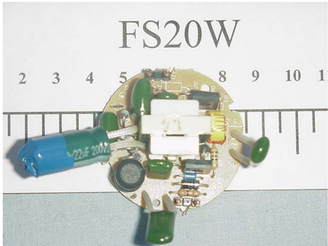
FIGURE 5 ENERGY SAVING LAMP (M/N: FS20W) MAIN BOARD (COMPONENT SIDE)
