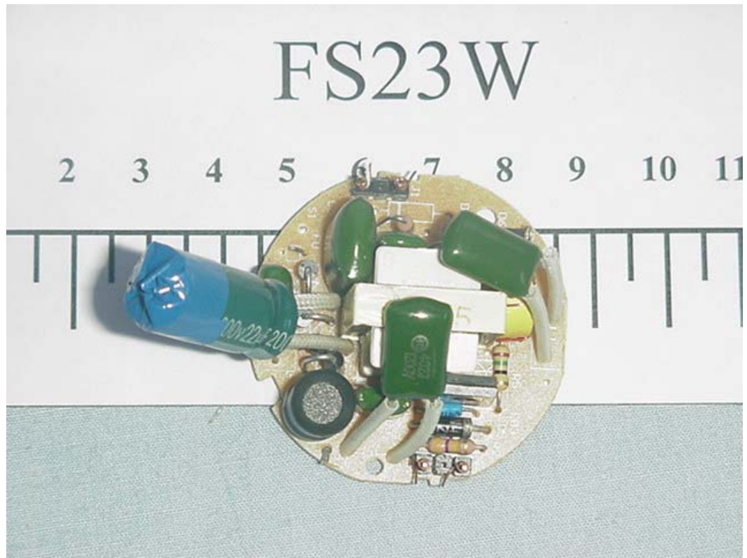
FIGURE 8 ENERGY SAVING LAMP (M/N: FS23W) MAIN BOARD (COMPONENT SIDE)
