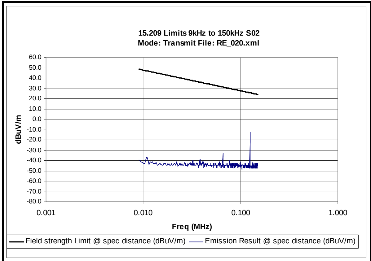
Radiated Spurious emissions 9kHz to 150kHz – Tx Mode 125kHz tag
