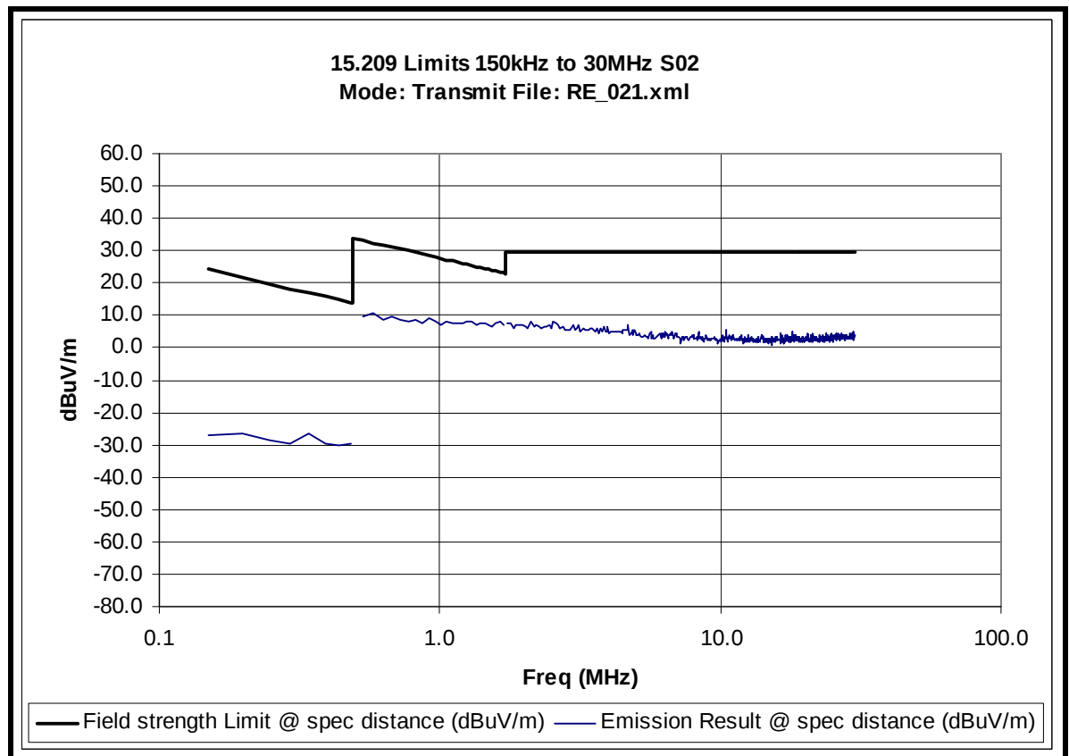
Radiated Spurious emissions 150kHz to 30MHz – Tx Mode 125kHz tag
