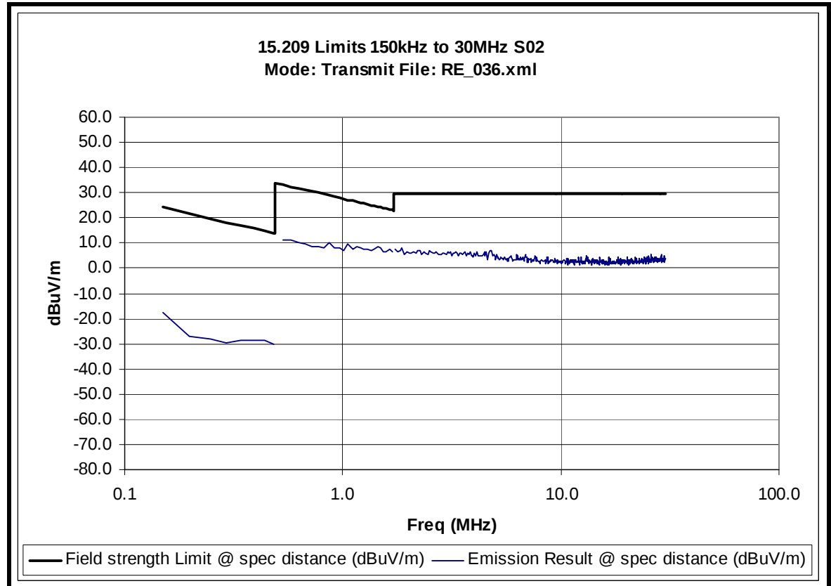
Radiated Spurious emissions 150kHz to 30MHz – Tx Mode 134kHz tag
