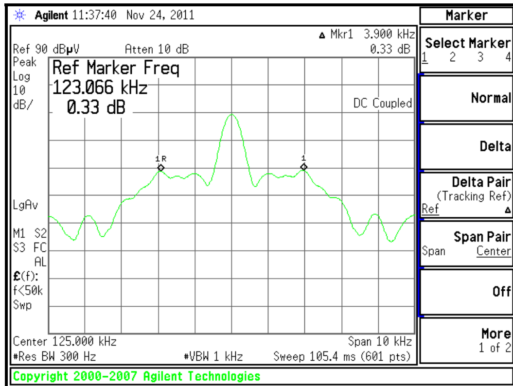
20dB Bandwidth- 125 kHz Tag
