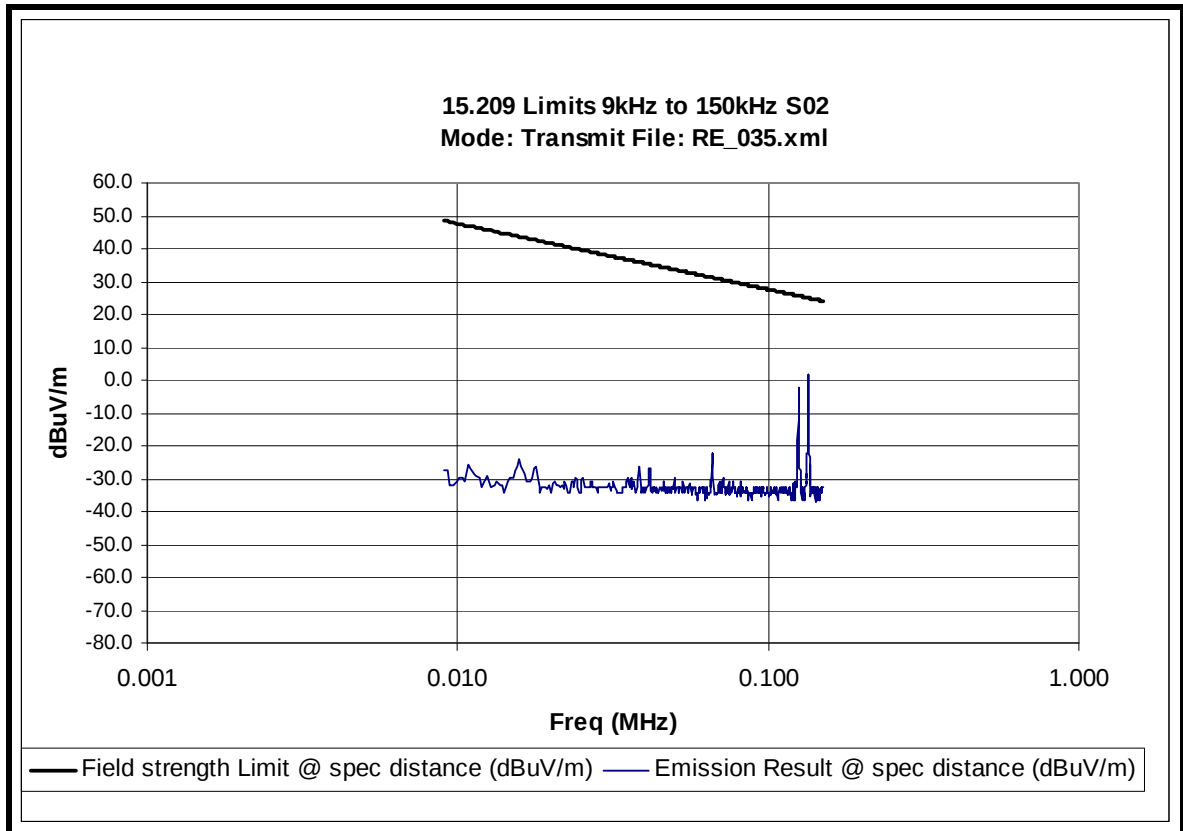
Radiated Spurious emissions 9kHz to 150kHz – Tx Mode 134kHz tag
