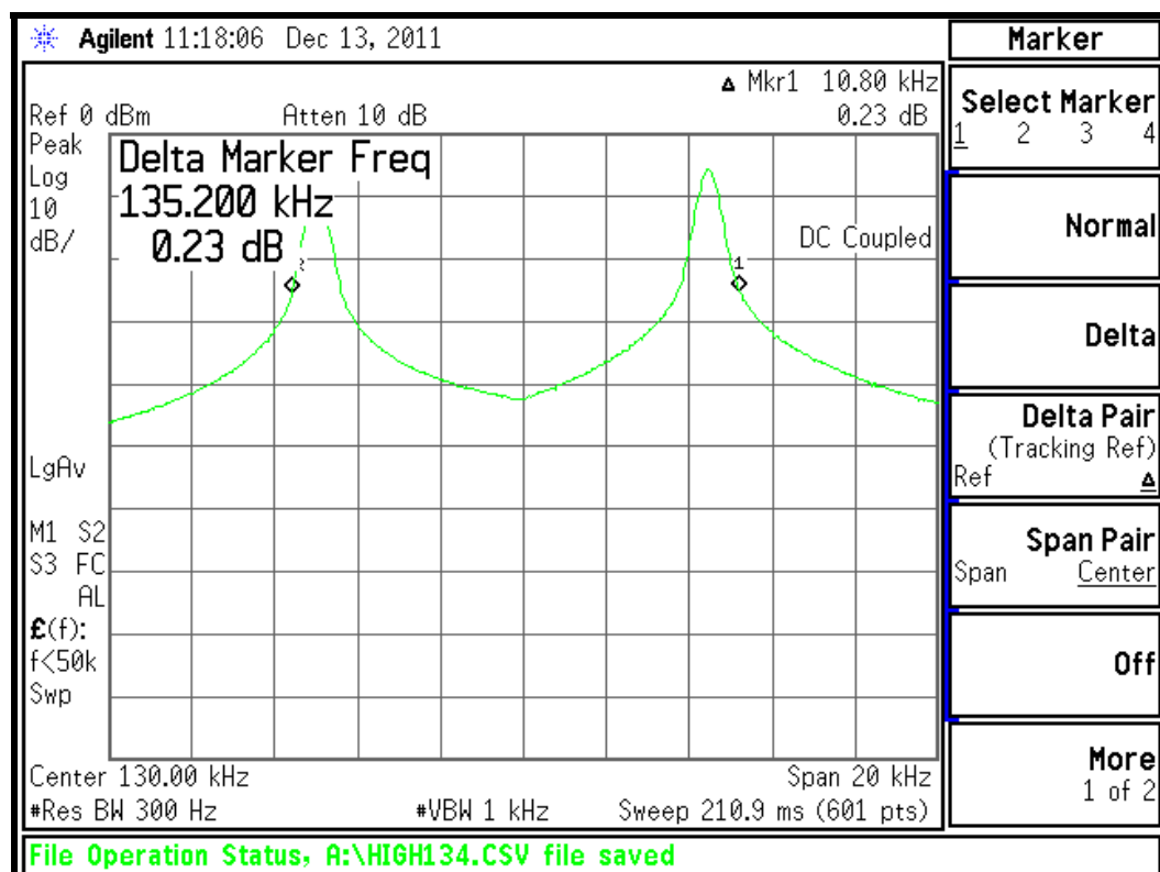
20dB Bandwidth - 134 kHz Tag
