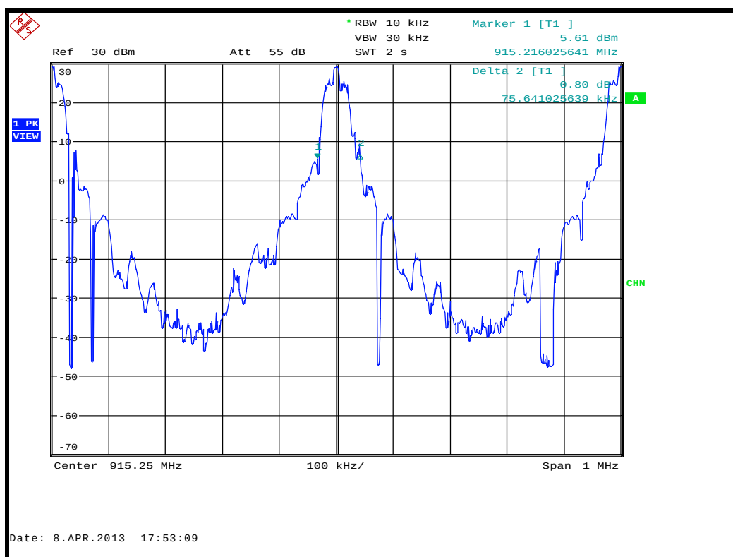
20dB Bandwidth
