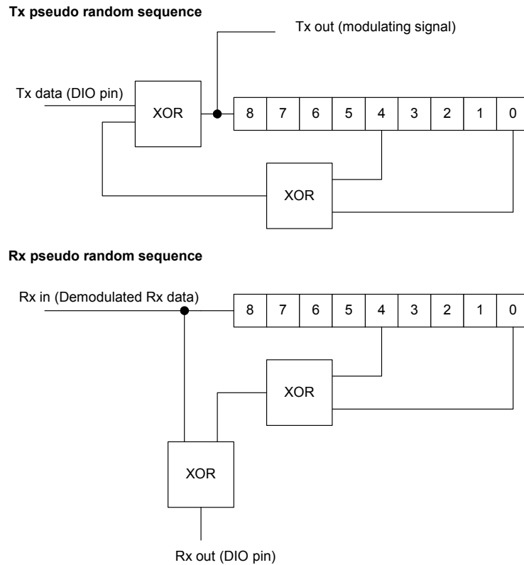
Figure 35. PN9 pseudo random sequence generator in Tx and Rx mode
