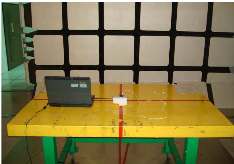
Above 1GHz _ Rear View _ MTK Module
