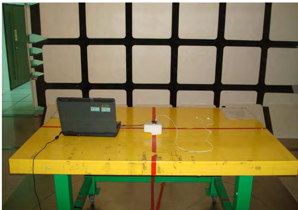
Below 1GHz _ Rear View _ MTK Module
