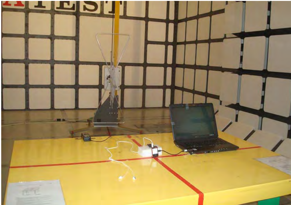
Below 1GHz _ Rear View _ CSR Module
