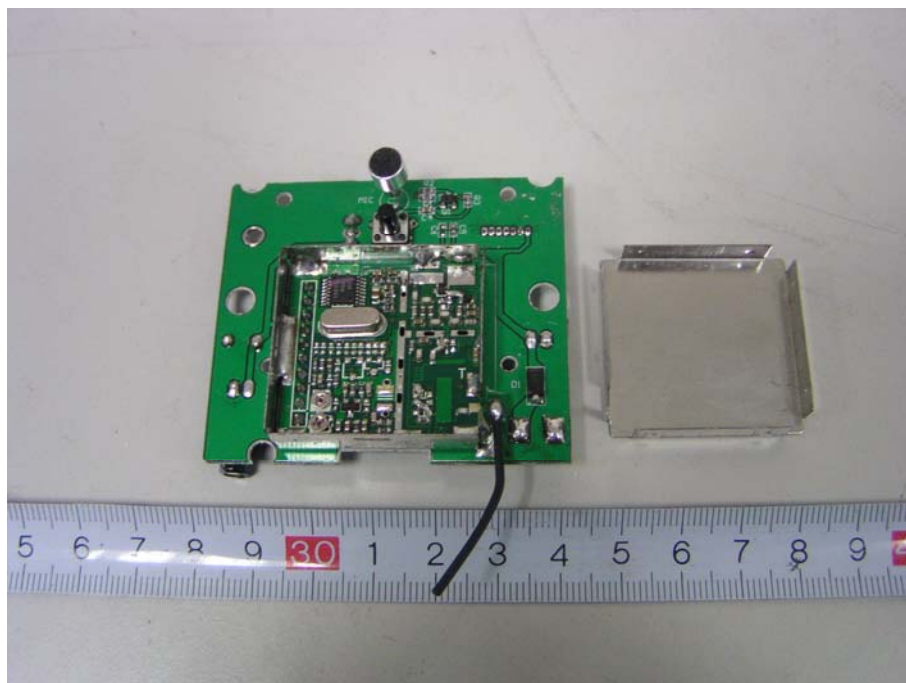
EUT – PCB 1 Unshielded Top View
