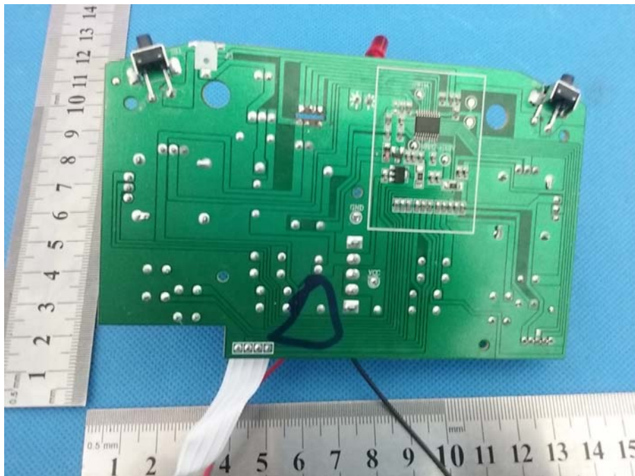
Model: K88 Photo 4
