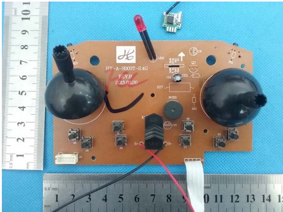
Model: K88 Photo 3
