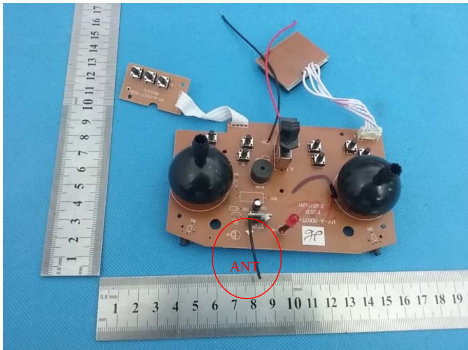
Model: K88 Photo 2
