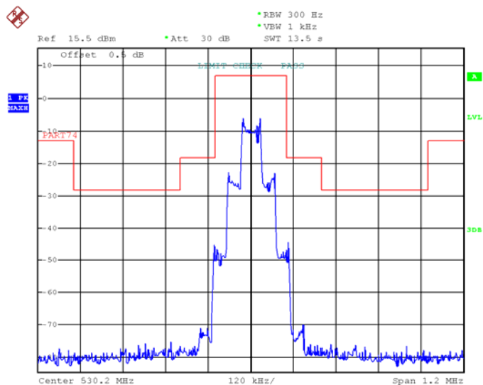
Emission Mask
