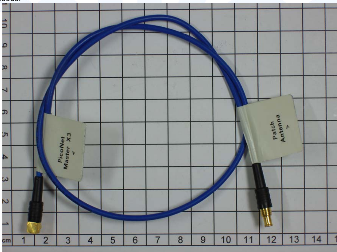
Antenna feeder
