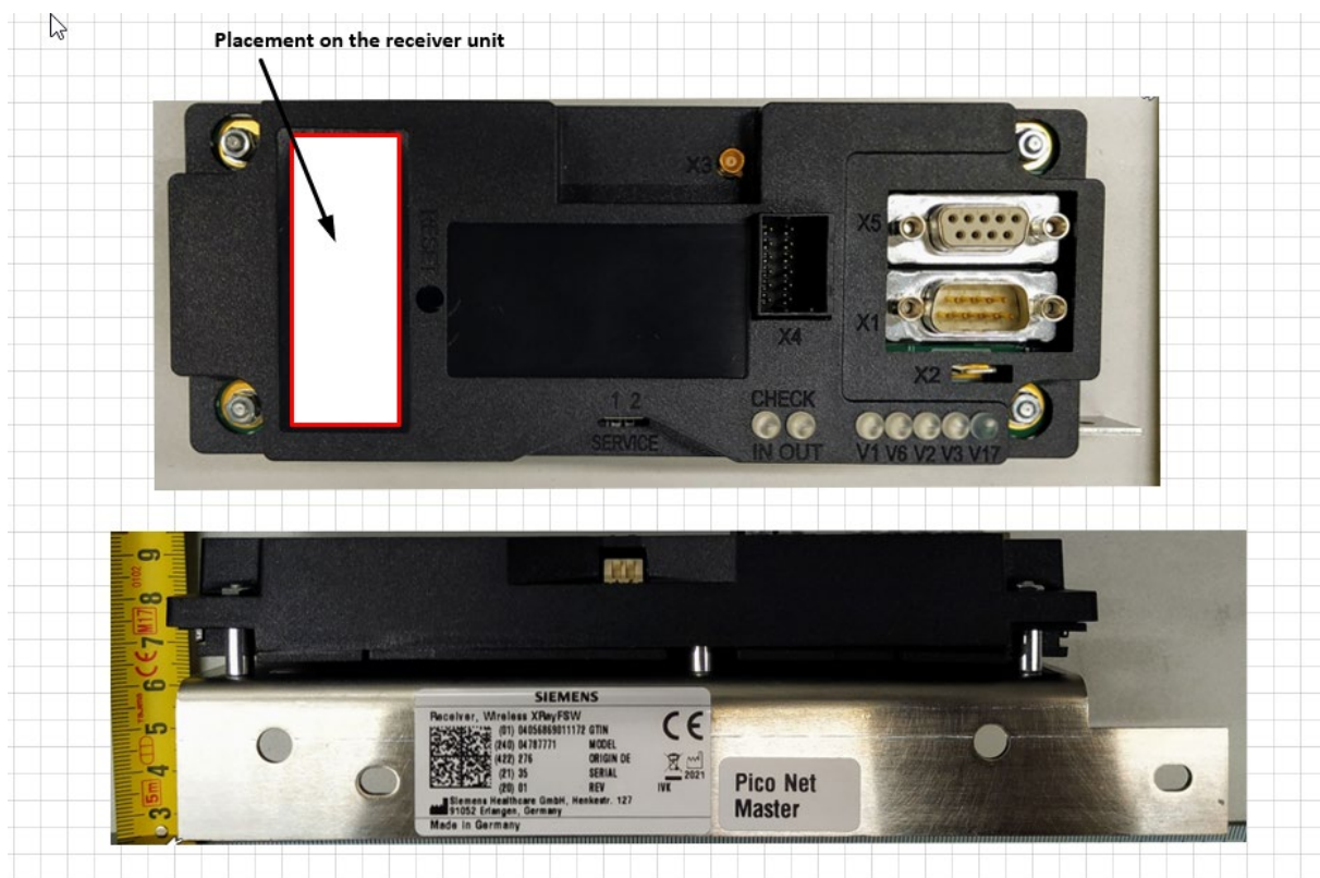
Figure 2: Label placement on Receiver the Wireless XRay Footswitch Model 04787771
