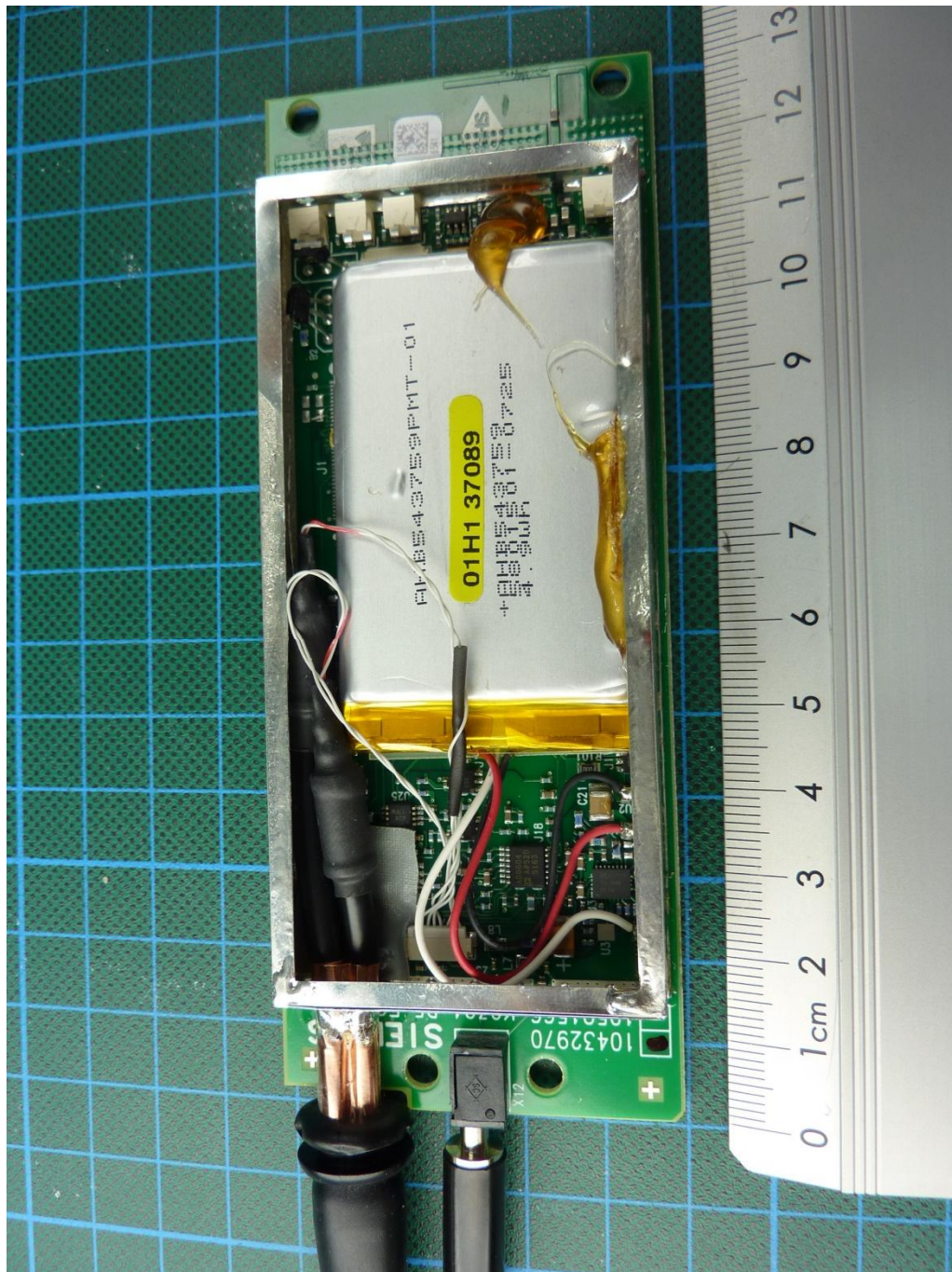
160125_6.JPG: PPU_098, PCB, top view, shielding opened
