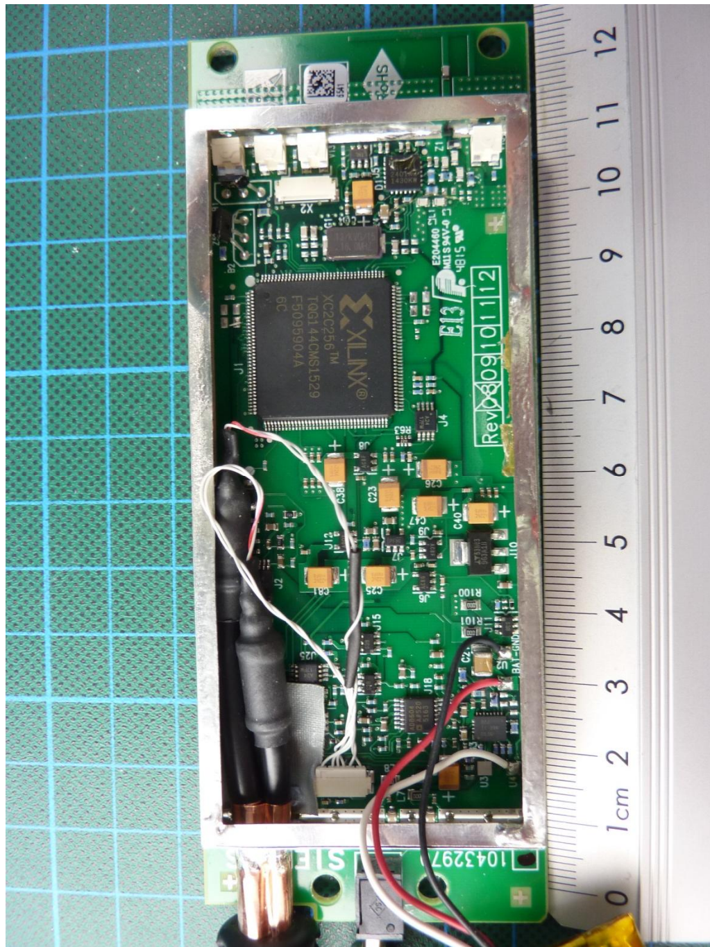
160125_7.JPG: PPU_098, PCB, top view, battery removed
