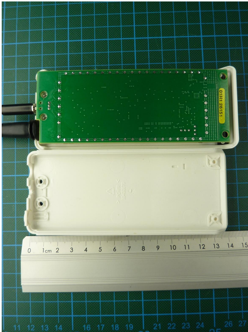
160125_3.JPG: PPU_098, internal view 1
