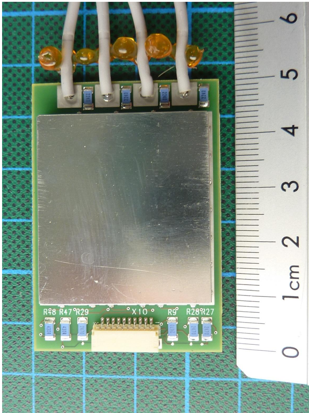
160125_107.JPG: PERU_098, preamp-PCB, top view
