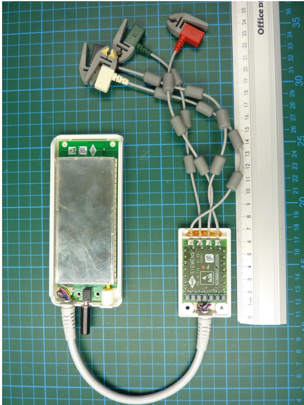
160125_104.JPG: PERU_098, internal view 1
