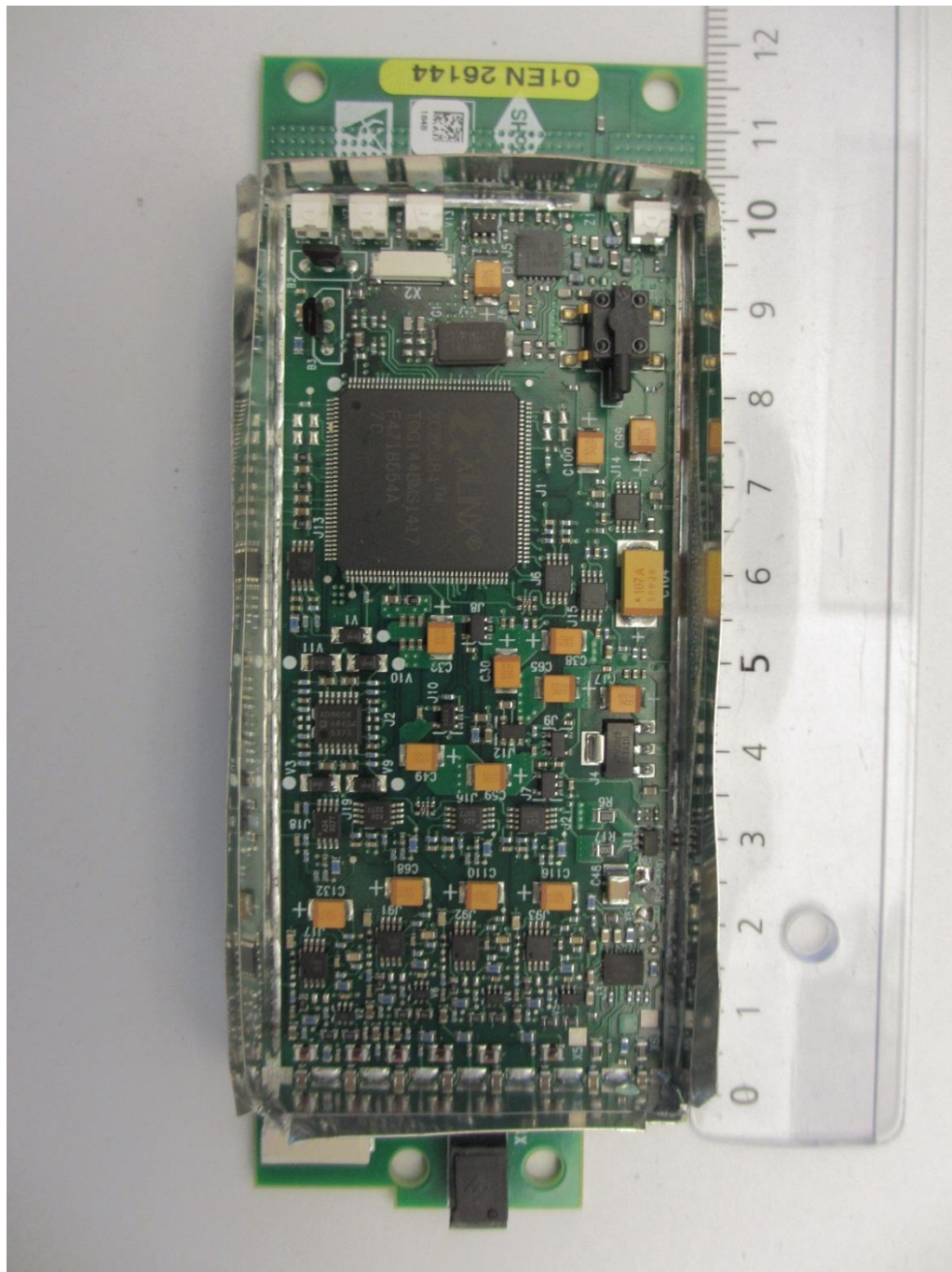
160125_114.JPG: PERU_098, PCB, top view, shielding and battery removed (supplied by the applicant)
