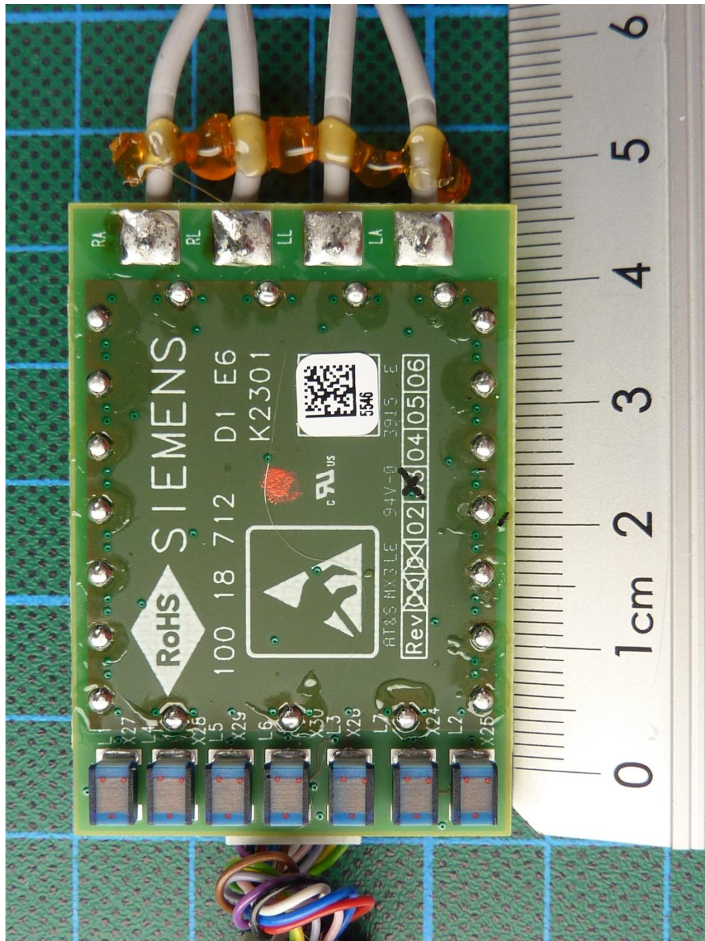
160125_106.JPG: PERU_098, preamp-PCB, bottom view
