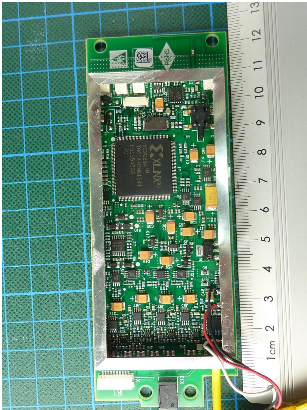
160125_112.JPG: PERU_098, PCB, top view, battery removed
