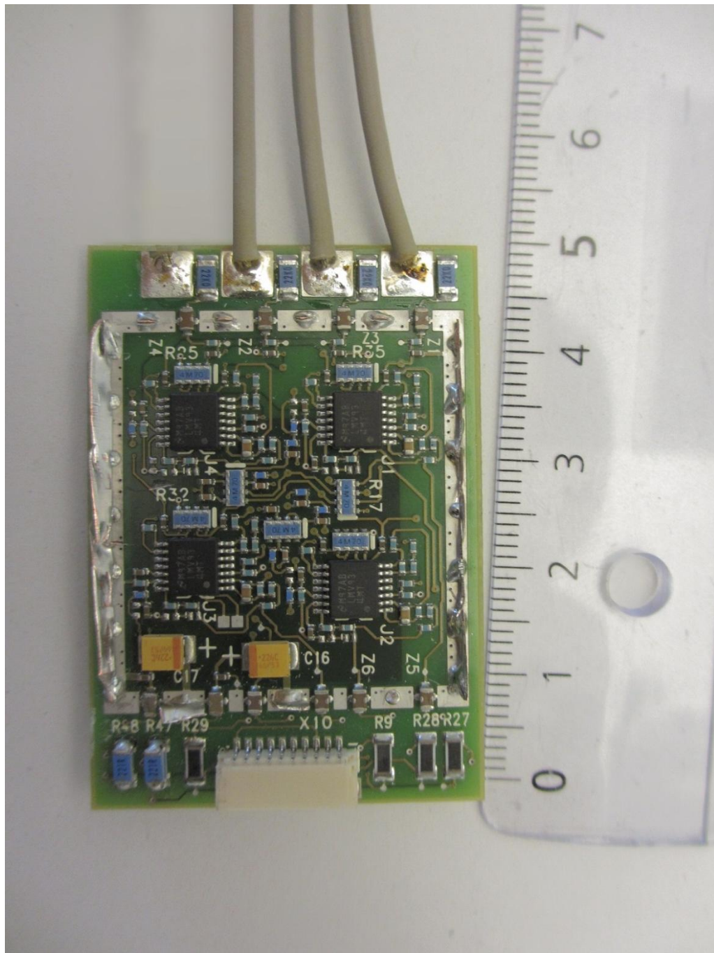
160125_113.JPG: PERU_098, preamp-PCB, top view, shielding opened (supplied by the applicant)
