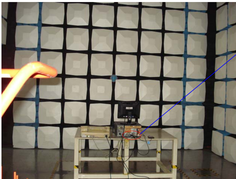
Spurious Emissions Test Setup - Rear View (Below 1GHz)
