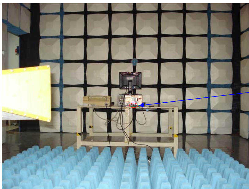
Spurious Emissions Test Setup - Rear View (Above 1GHz)
