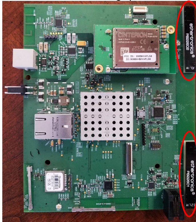
Satellite Tracking of People Modem Module board and Antenna locations. The Antennas are circled.
