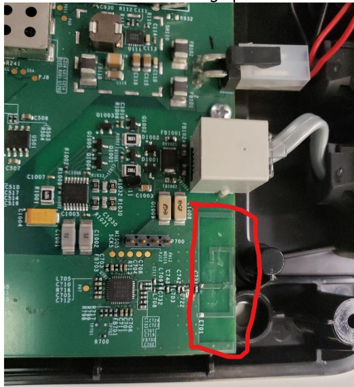
Wi-Fi Antenna
