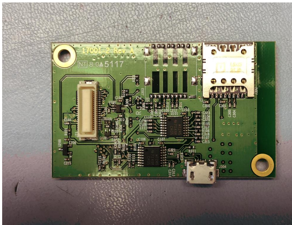
Satellite Tracking of People Modem Module board
