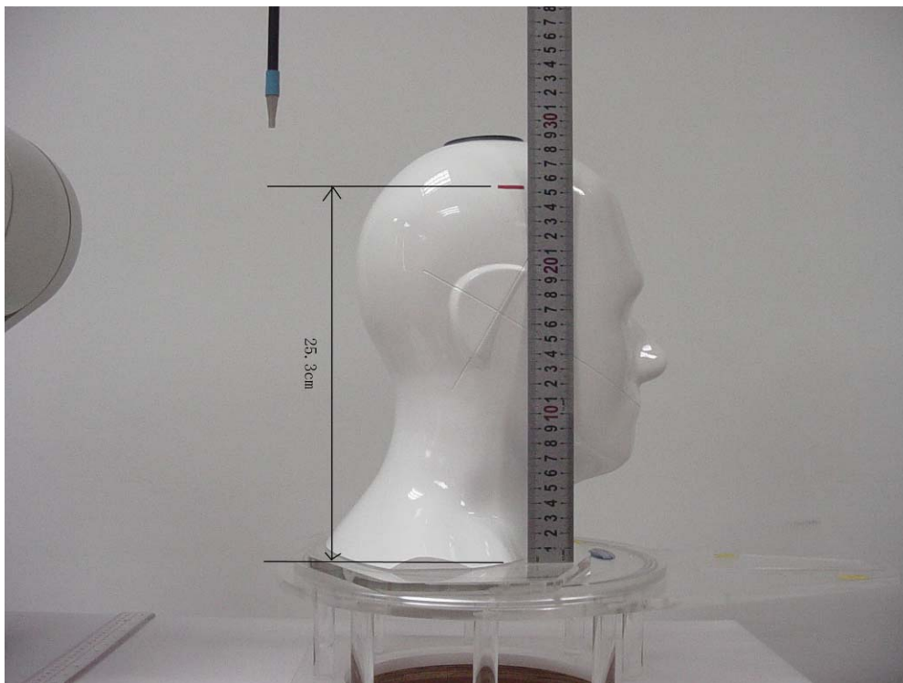
Fig.2 SARA2 System Test Layout
