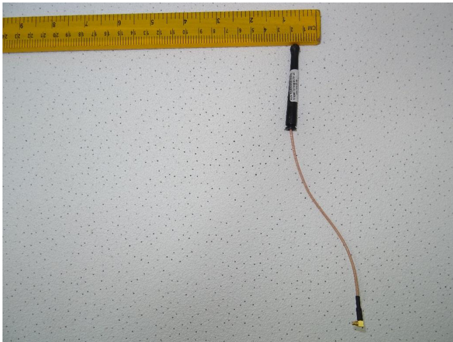
Antenna 1: Centurion MAF94152 Omni antenna (-2 dBi)
