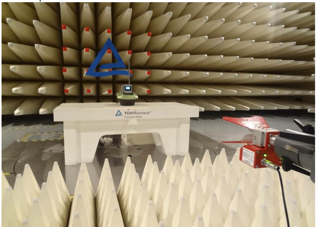
Test setup
