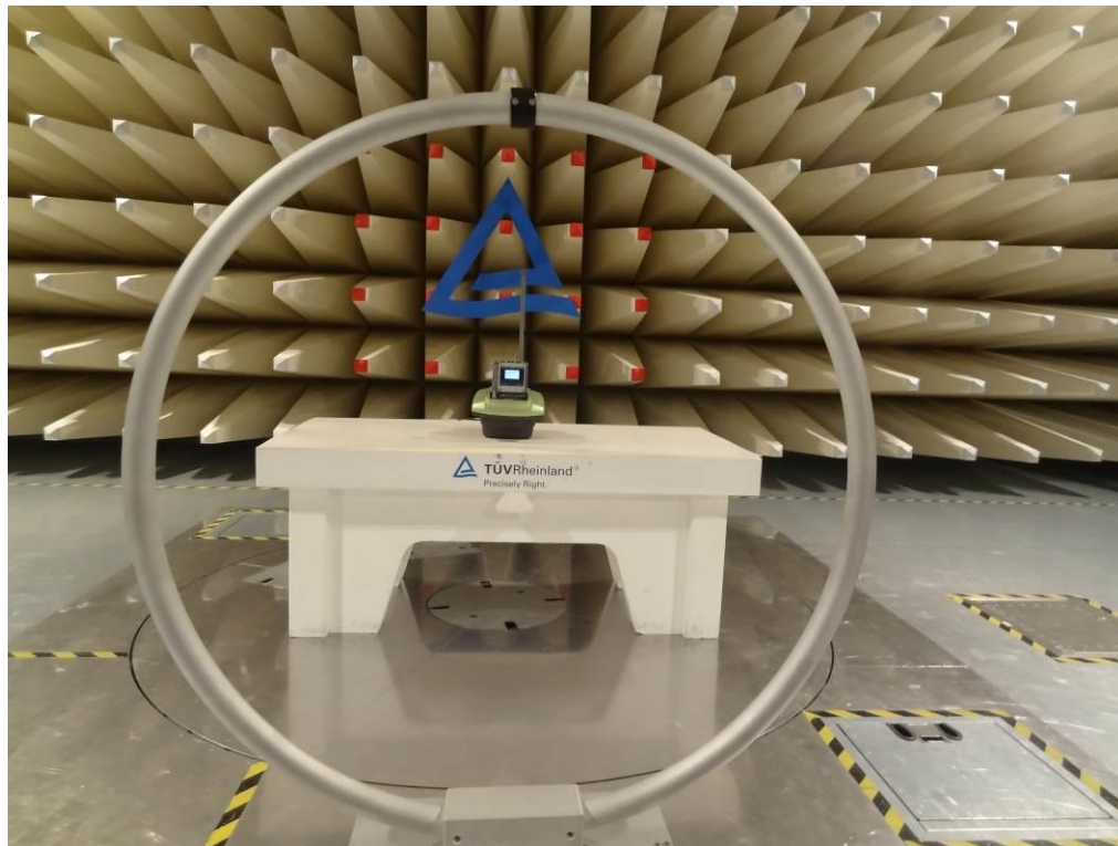
Test setup
