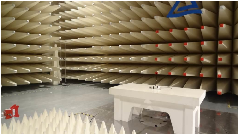
Radiated Test setup
