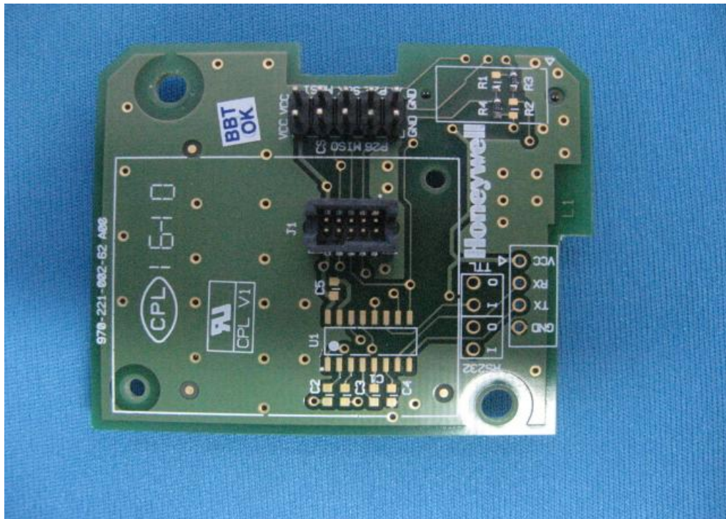
EUT Bottom layer's Top View
