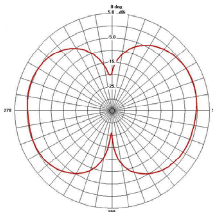
Elevation Plane WCP2400MMCX
