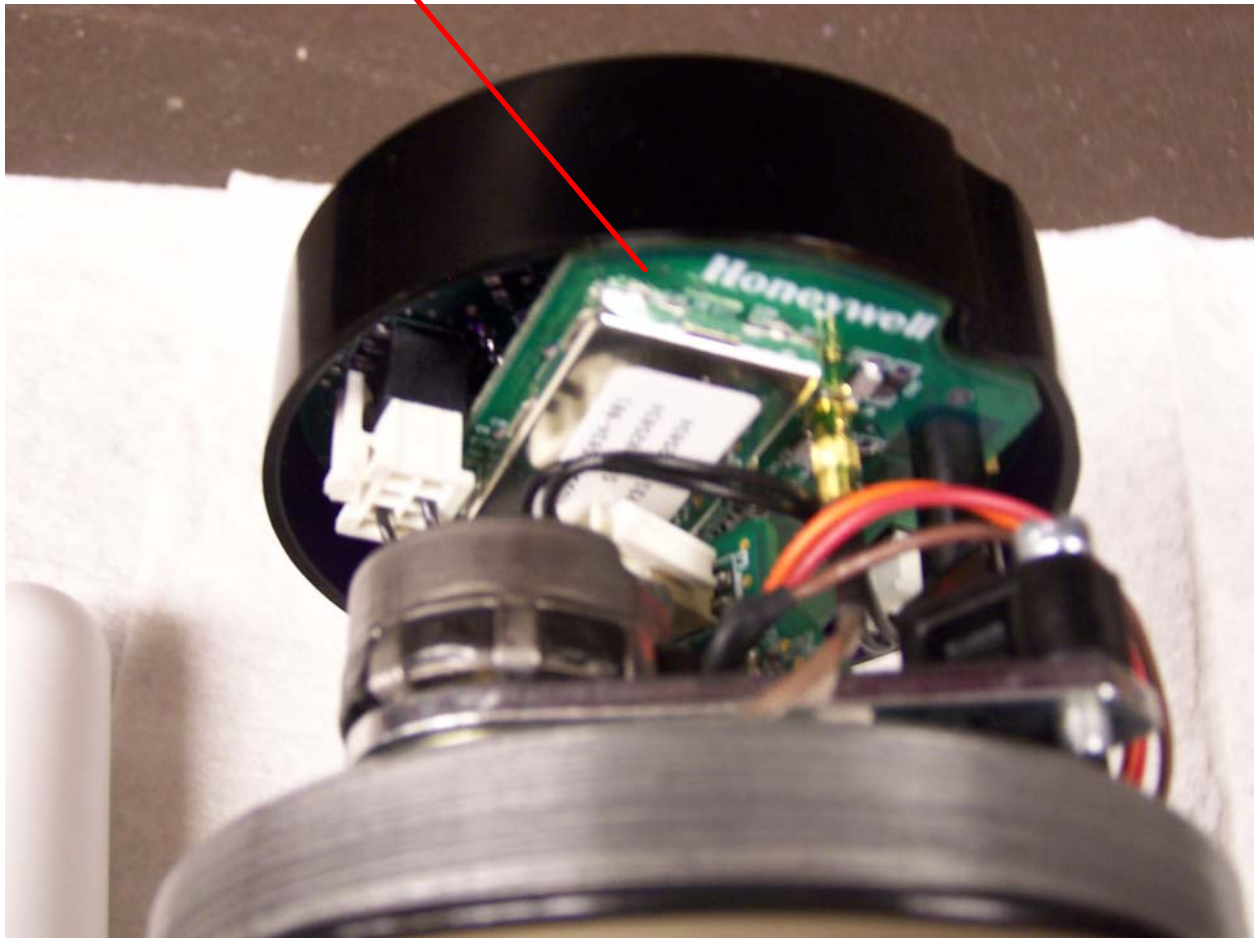
WCX1 – RADIO BOARD
