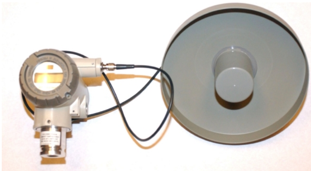
XYR 6000 WIRELESS TRANSMITTER WITH REMOTE MOUNTED UNIDIRECTIONAL 14 dBi ANTENNA, HYPERLINK TECHNOLOGIES HGV-2414D HONEYWELL P/N 50018415-001
