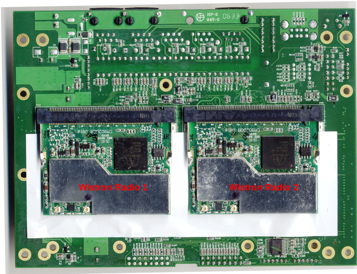
Figure 3: 3eTI System Board, showing Wistron radio modules.
