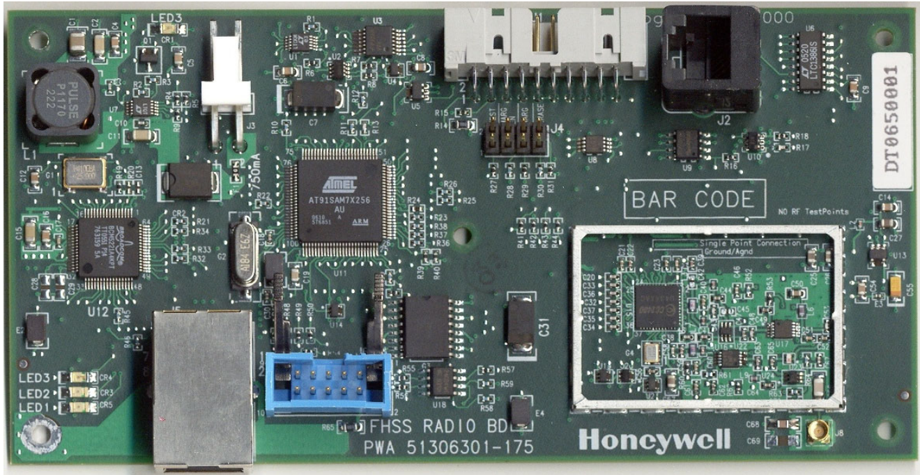
Figure 2: Honeywell FHSS radio side A without RF shield
