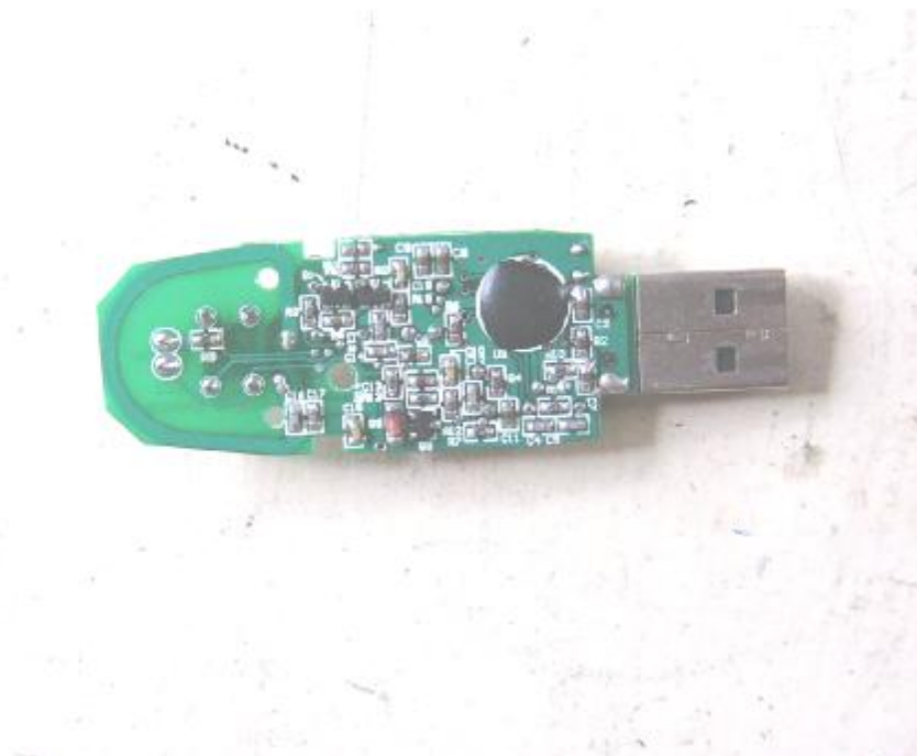
Rx board solder side
