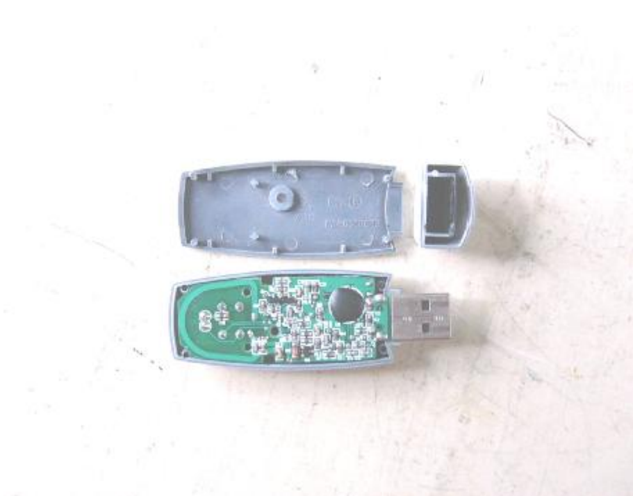
Rx inside whole view
