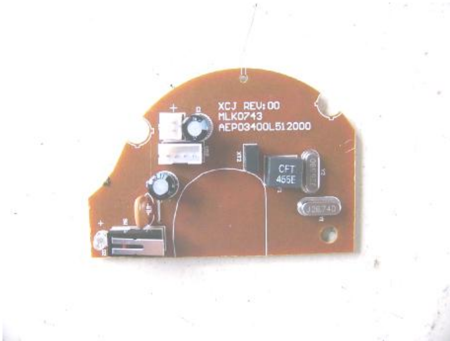
Rx board component side
