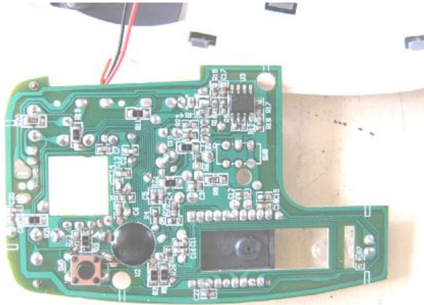
Main board solder side
