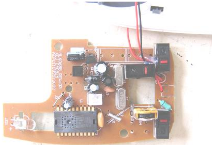
Main board component side
