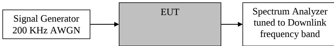
Figure 7: Test setup for downlink noise power measurement in the presence of a downlink signal
