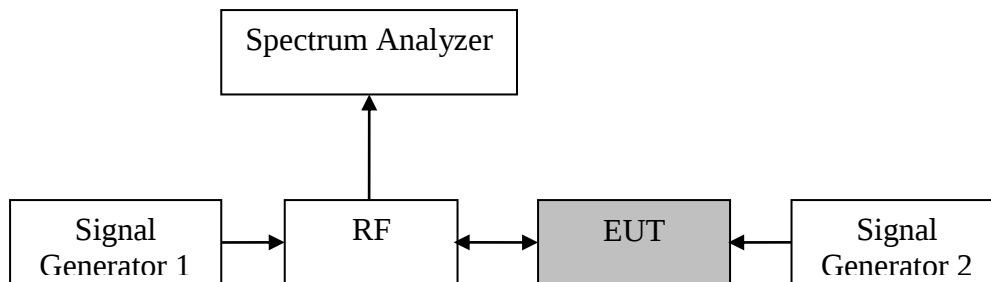
Figure 10: Variable uplink gain test setup
