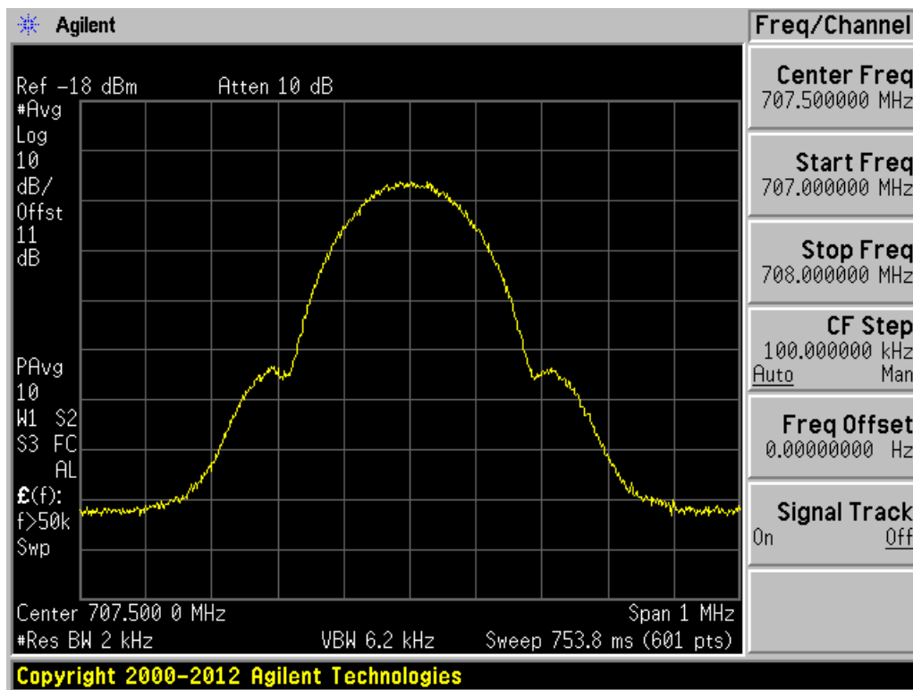
Uplink, Band 12 &amp; 17, GSM Input.
