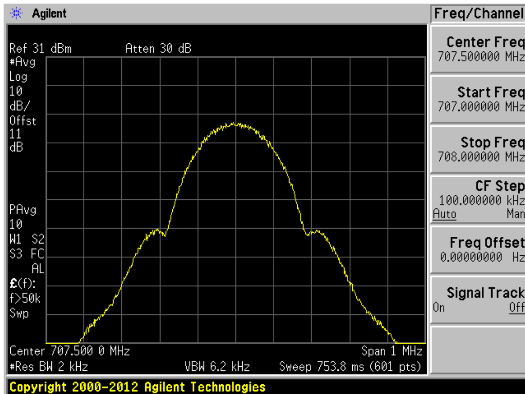
Uplink, Band 12 &amp; 17, GSM Output.
